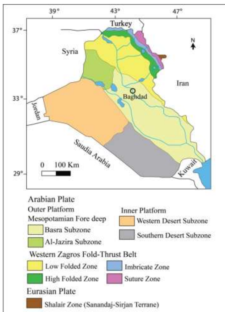
Fig. 2: Tectonic divisions of Iraq showing the studied area [1] and [8].
