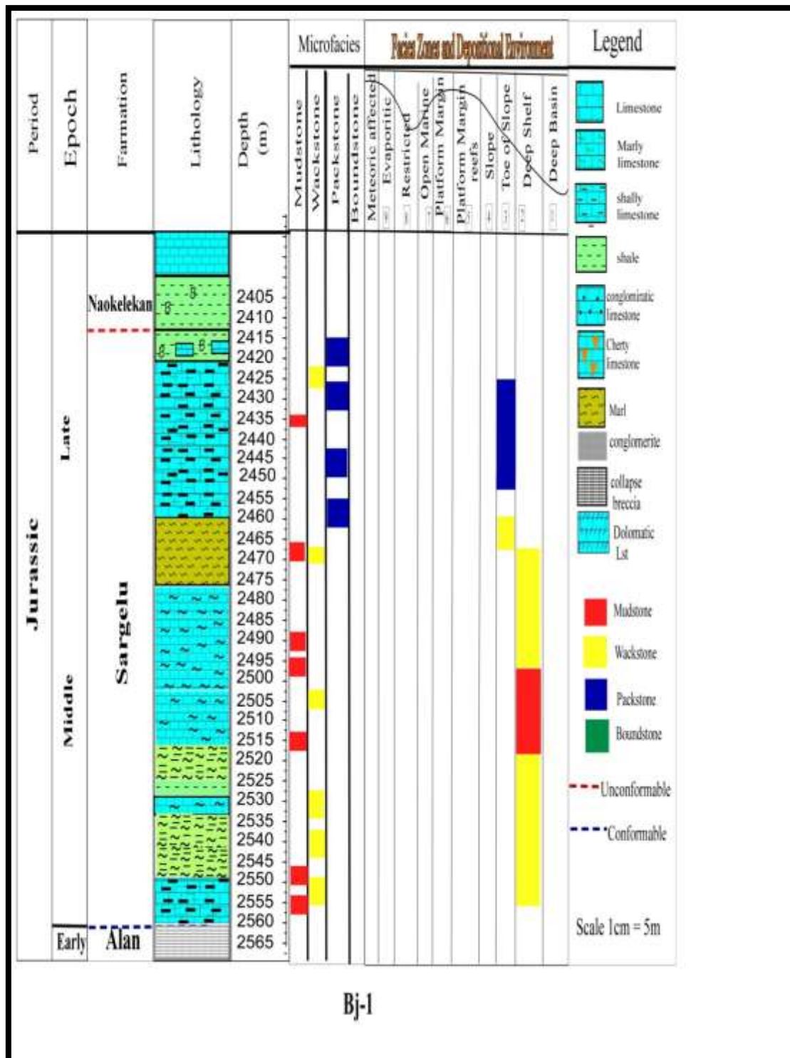
Fig. 5: Microfacies &amp; environment zones distribution, Bj-1 Well.
