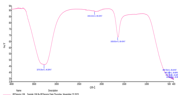
Figure 3. FT-IR Spectrum of Ciprofloxacin (CIP)
