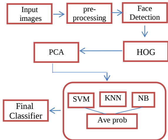
Fig. 1. Overview Of Facial Expression System
