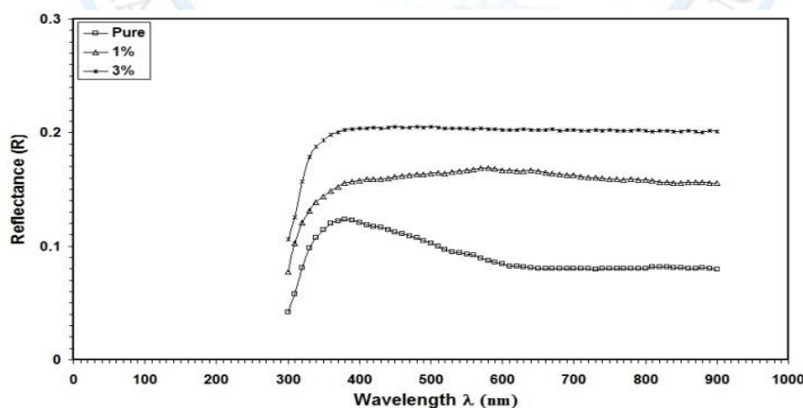
Fig. (2): Reflectance versus wavelength for pure and kaolin doped PVA films (b) After irradiation
