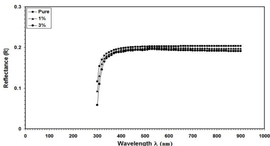
Fig. (2): Reflectance versus wavelength for pure and kaolin doped PVA films (a) Before irradiation
