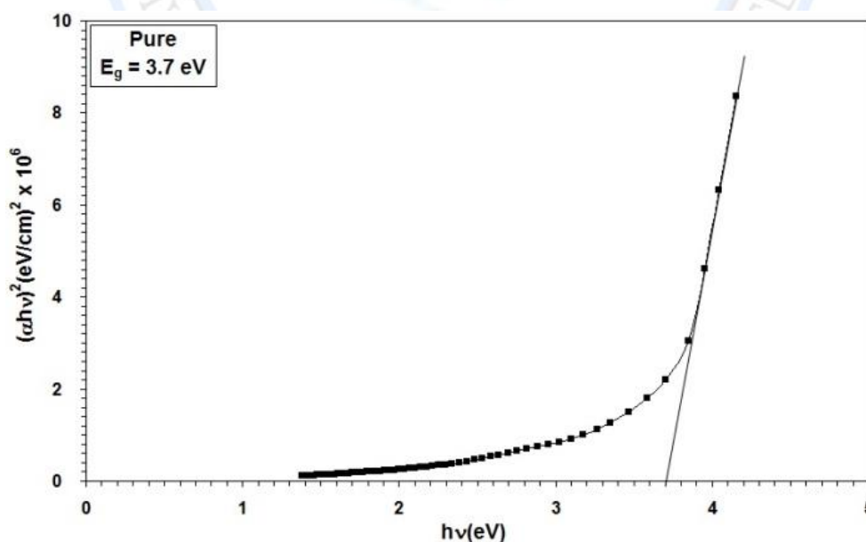
Fig (3) (\alpha h\nu)^2 for pure PVA films : (a) Before irradiation
