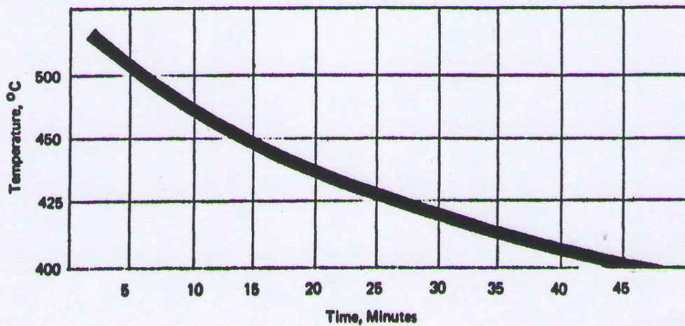
Fig. ( 2 ) Sealing time vs temperature of solder glass
