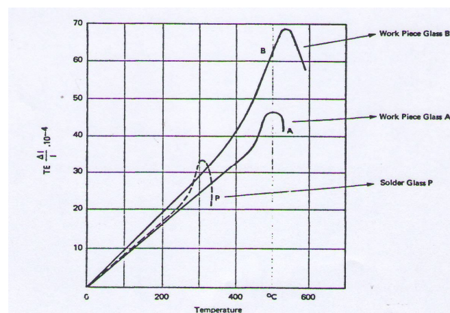
Fig. ( 5 ) Thermal expansion of solder glass
