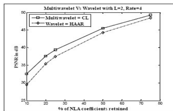
Figure (4): Comparison of PSNR values for IDMWT and MVSQ-IDMWT for 'Tiger' image
