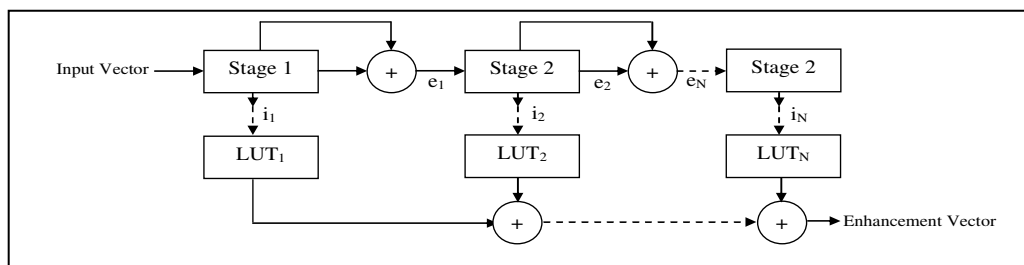
Figure(1): Multistage Vector Quantization System
