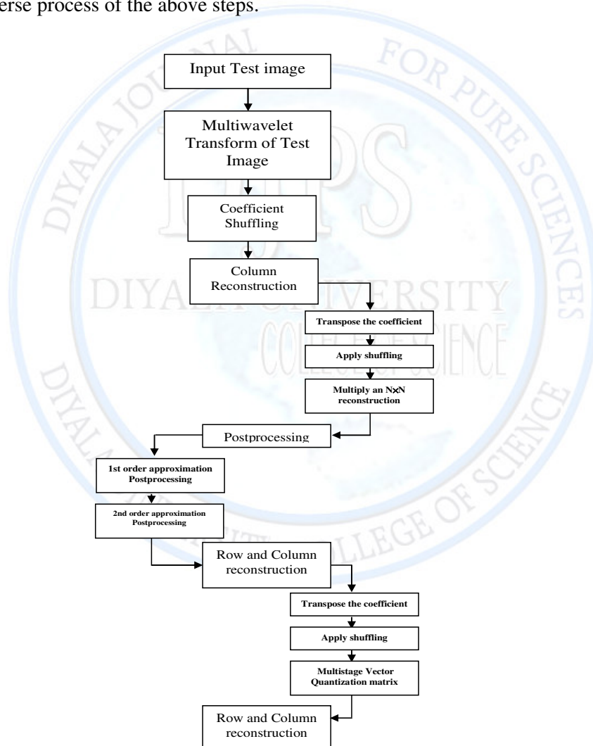
Figure (2): Block Diagram of proposed algorithm
