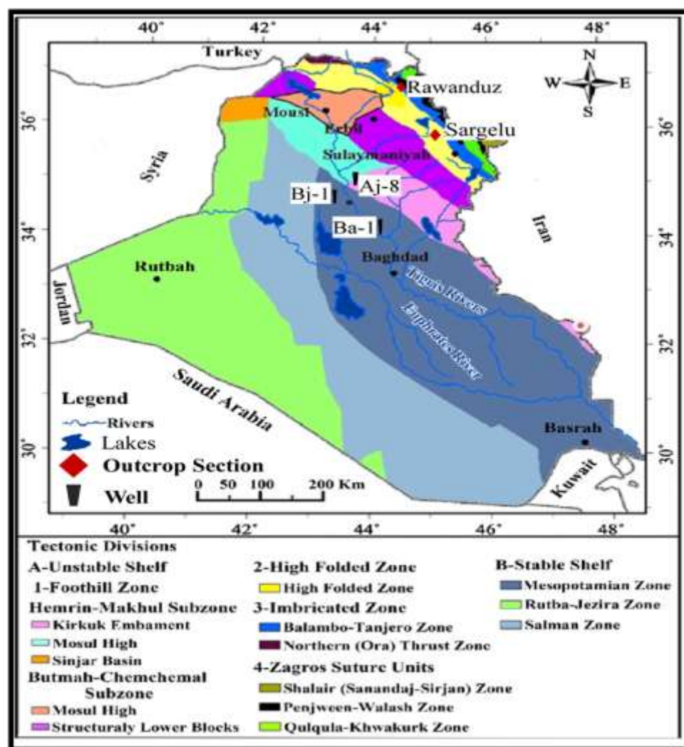
Fig.1: Tectonic zones of Iraq showing the study area (modified from Al-Zubaydi et al.[14]).
