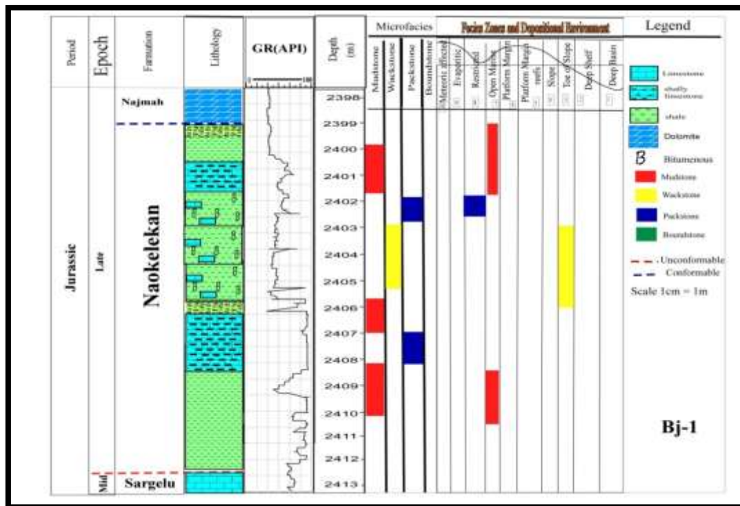
Fig. 3: Microfacies &amp; environment zones distribution, Bj-1 Well.
