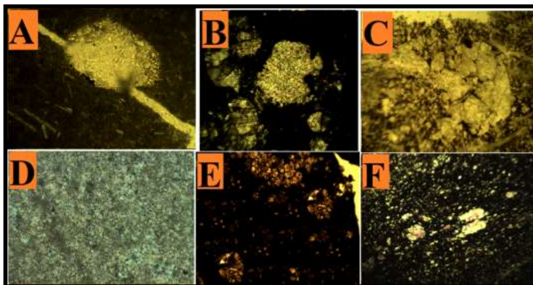
Plate.1: A, Druzy mosaic cement, in micritic matrix, in lower part of well Bj-1, P.L. (X10). B, Syntaxial rim cement in upper part of well Aj-8, P.L. (X10). C, Blocky Cement, consists relatively of large anhedral to subhedral calcite crystals, P.L. (X40). D, Neomorphism, partially recrystallization of micrit, P.L. (X10). E, Spotted mosaic fabric in lower part of well Ba-1, P.L. (X10). F, Aphanitic texture in the Lime-Packstone Microfacies.
