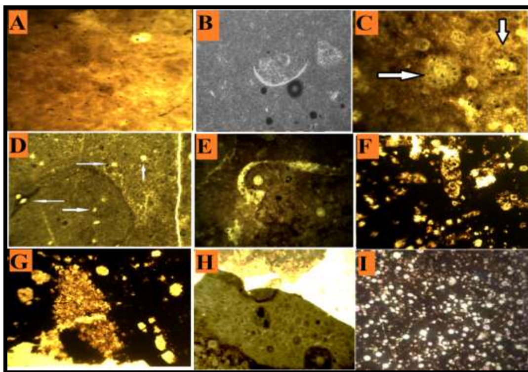
Plate 3: A, Non-fossiliferous lime mudstone submicrofacies in well Ba-1, P.L. (X10). B, Bioclastic lime mudstone submicrofacies in well Ba-1, P.L. (X10). C, Benthonic foraminifera in the lime-wackestone microfacies in well Aj-8, P.L. (X40). D, Calcisphere filled with calcite, in the lime-wackestone microfacies in middle part of well Ba-1, P.L. (X10). E, Pelecypod in micrite matrix affected by dissolution and made up of secondary porosity filled with sparry calcite (granular cement), in the lime-wackestone microfacies in upper part of well Aj-8, P.L. (X40). F, G, Bioclasts in the lime-packstone microfacies in upper and lower parts of well Ba-1 P.L. (X10)., H, Peloids in the lime-packstone microfacies, in lower part of well Bj-1, P.L. (X10). I, Calcisphere in the lime-packstone microfacies.
