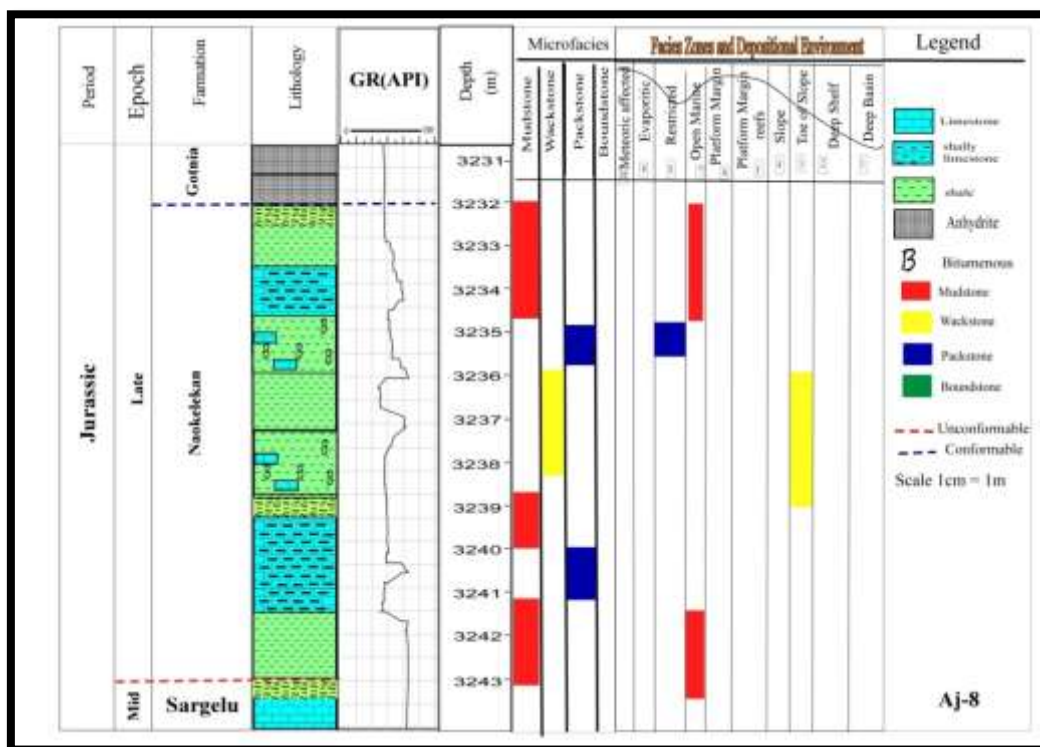
Fig. 2: Microfacies & environment zones distribution, Aj-8 Well.
