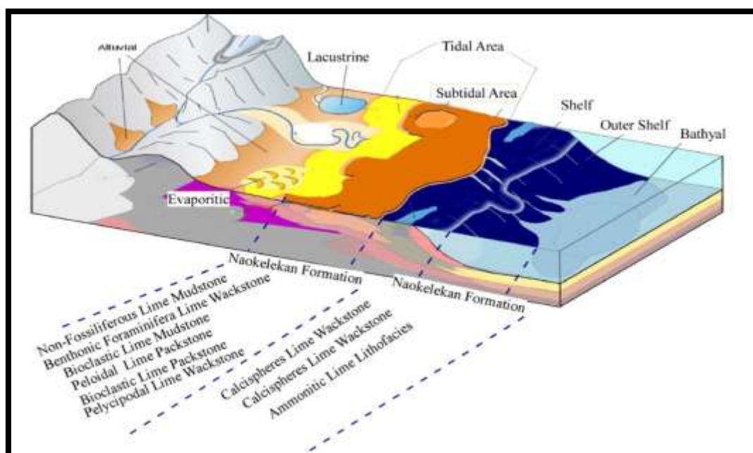
Fig. 5: Depositional model of Naokelekan Formation.
