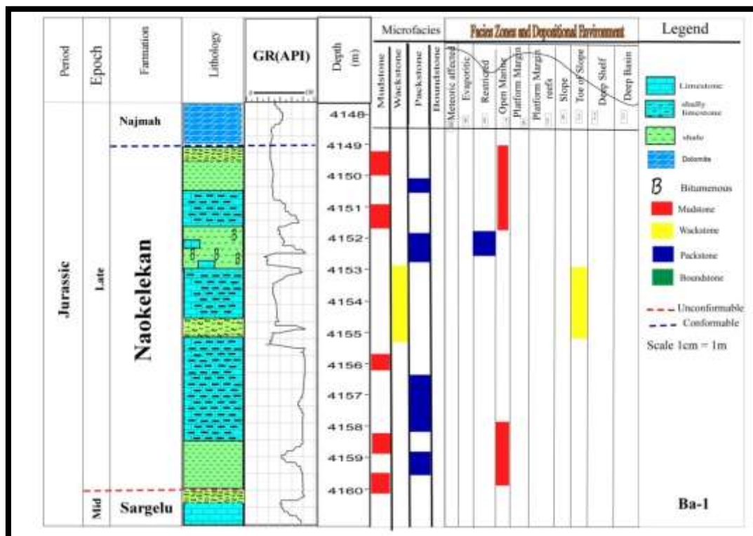
Fig. 4: Microfacies &amp; environment zones distribution, Ba-1 Well.
