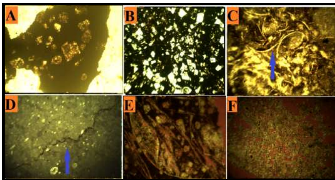
Plate 2: A, Contact rhomb fabric, in micritic matrix, in lower part of well Ba-1, P.L. (X10). B, Floating rhombs fabric in middle part of well Bj-1, P.L. (X10). C, Physical compaction, tangential contact between particles, P.L. (X10). D, Irregular stylolites in lower part of well Aj-8, P.L. (X10). E, Interparticle porosity in the Lime-Packstone Microfacies. F, Vuggy porosity in lower part of well Bj-1, P.L. (X10).
