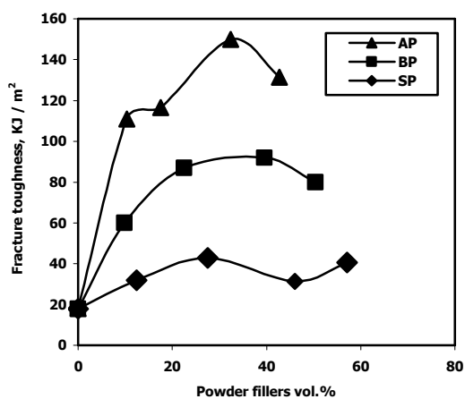
Fig. 8: Influence of powder fillers volume fraction on the fracture toughness of novolac.
