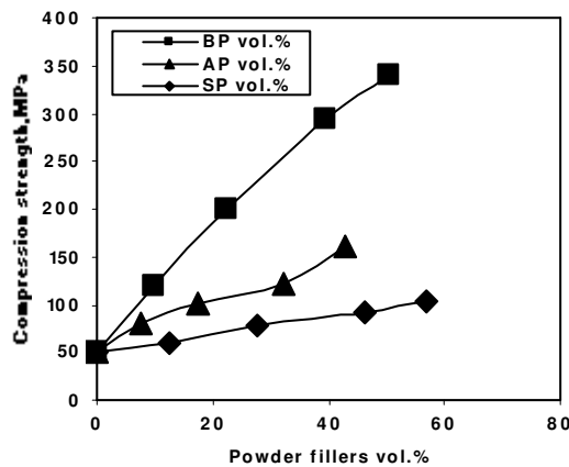
Fig. 4: Influence of powder fillers vol.% on the compression strength of PFN.
