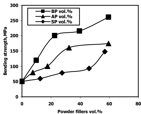
Fig. 6: Influence of powder fillers vol.% on the bending strength of PFN.
