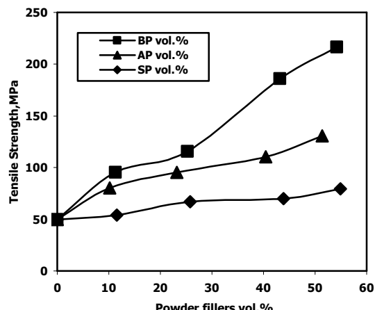
Fig. 2: Influence of powder fillers vol.% on the tensile strength of novolac.
