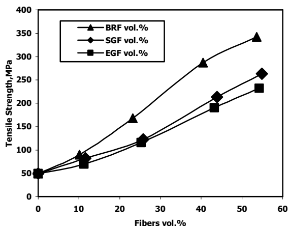
Fig. 1: Influence of fibers vol.% on the tensile strength of novolac.
