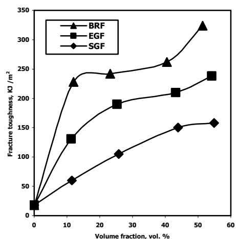
Fig. 7: Influence of fibers volume fraction on the fracture toughness of novolac.
