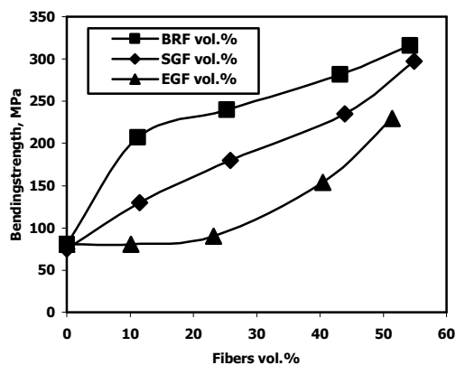
Fig. 5: Influence of fibers vol.% on the bending strength of PFN.
