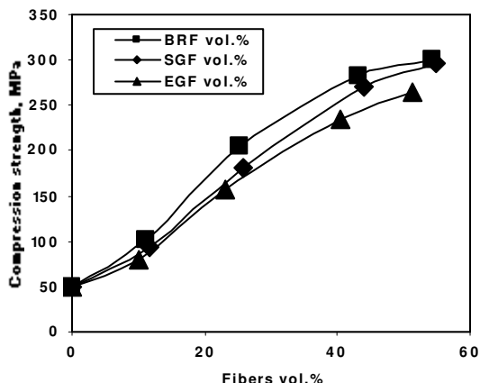
Fig. 3: Influence of fibers vol.% on the compression strength of PFN.
