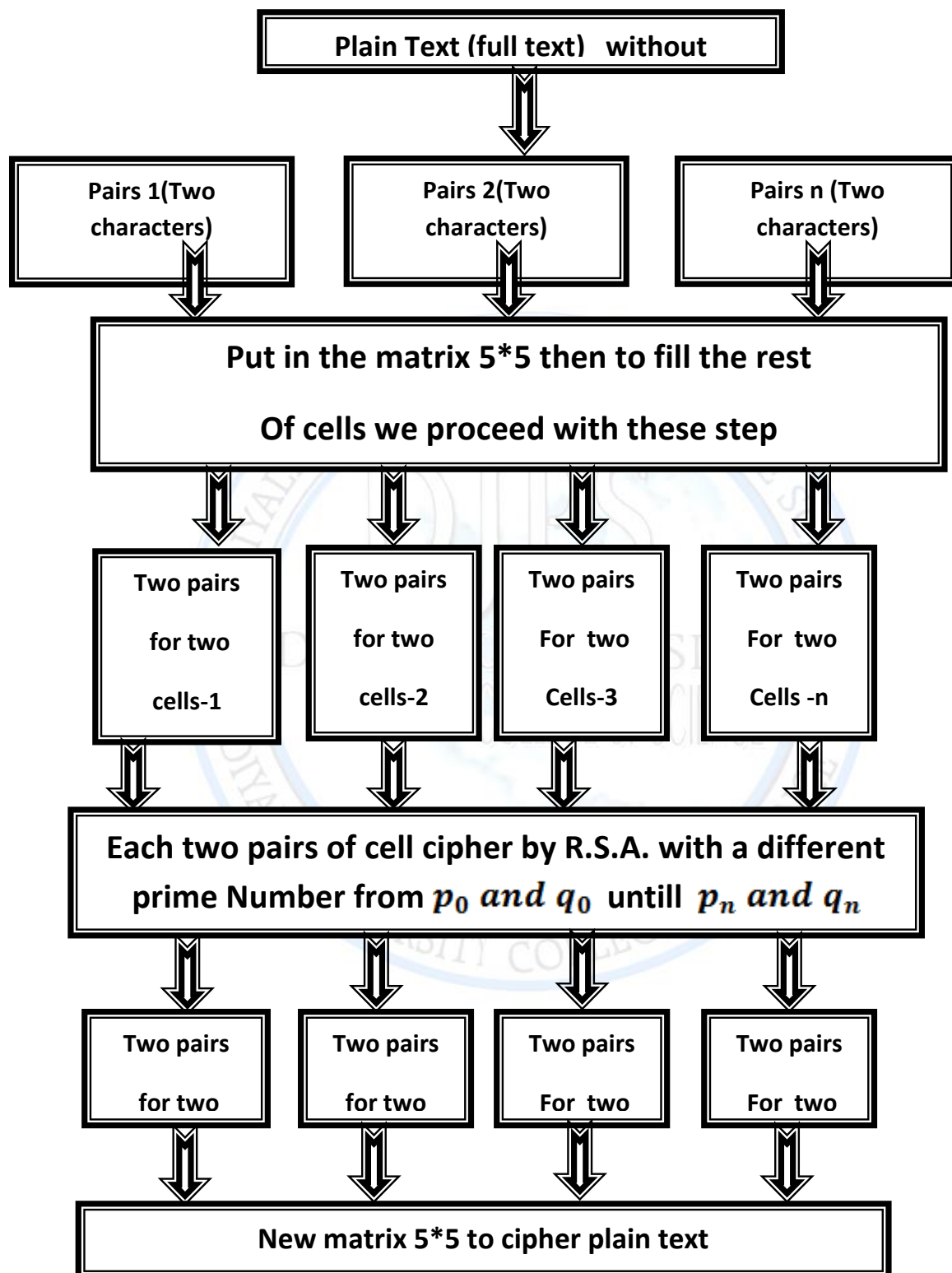
Fig (2) Mixed Algorithm
