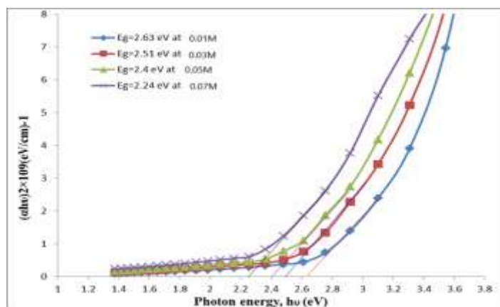
Fig. 8: values of (\alpha h\nu)^2 with the incident photon energy of (CdO) films at different molar concentrations in the deposition
