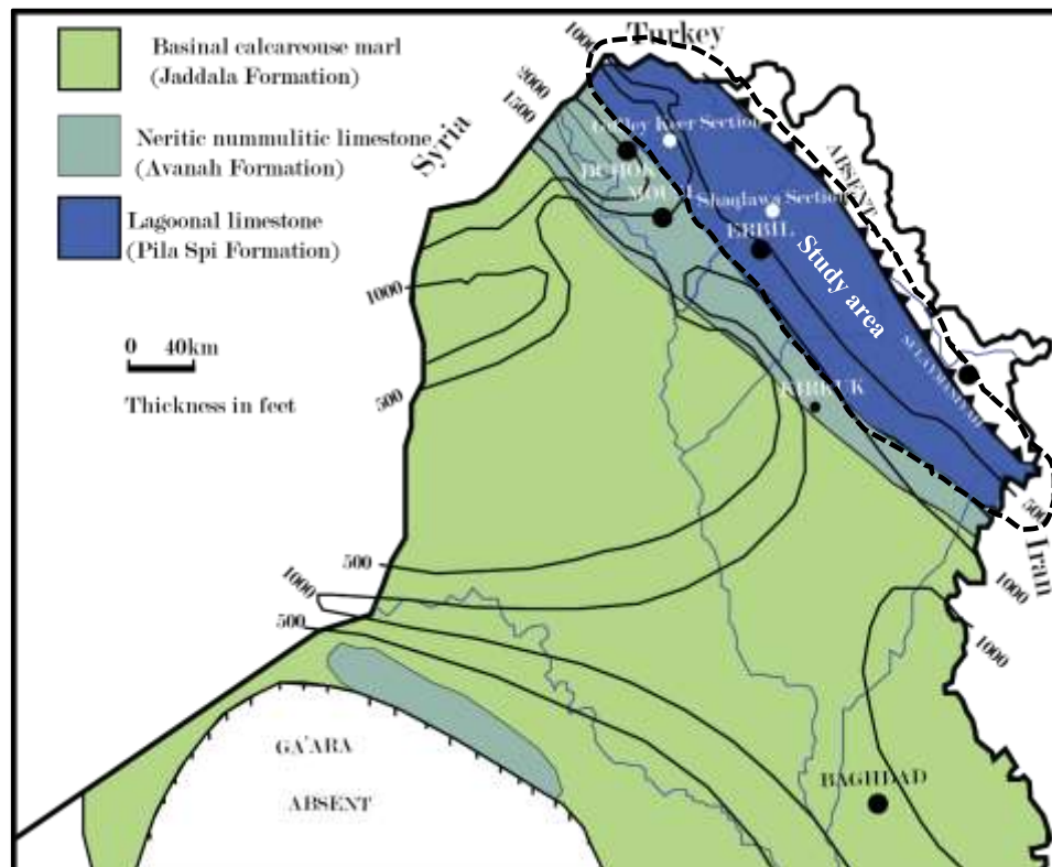
Fig. 2: Isopach facies map of the Middle-Upper Eocene showing distribution of lagoonal limestone (Pila Spi Formation), limestone (Avanah Formation), and Basinal marl (Jaddala Formation) (modified after [2]).
