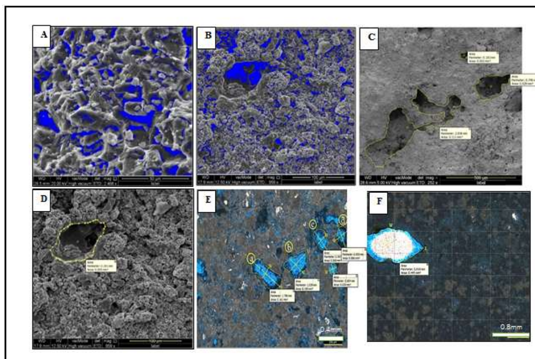
Fig. 5: SEM photograph of some studied thin sections. (A) Intercrystalline and micro-vugs porosity, the value of porosity is 12%. (B) The moldic porosity with a value of 13% (C) The vugs porous, the pore size ranges between Micropore-Mesopore. (D) The vugs porosity, pore size is in range Micropore-Mesopore (Large). (E) The pores size is Mesopore (Small) P.P.L, (4X), B.R. (F) The pores size is Micropore-Mesopore P.P.L, (4X), B.R.
