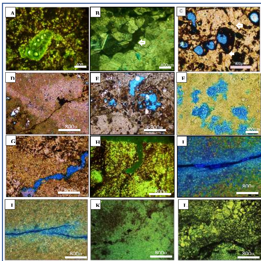
Fig. 4: Thin section photos for porosity types from Pila Spi Formation. (A) Intraparticle porosity of skeletal grain formed by leaching of soft parts with skeleton. P.P.L (4X), GK. 11, N.R. (B) The intercrystalline porosity within collected mosaic crystals of blocky cement (arrow) P.P.L (4X), SA.23, B.R. (C) Moldic porosity formed by partly leaching of some grains, partly filled by bitumen from the upper part of Pila Spi Formation P.P.L (4X), GK. 38, B.R. (D) Microfracture porosity occur along the fracture by leaching or dissolution within micrite matrix filled with bitumen P.P.L (4X), GK. 21, B.R. (E) Interparticle porosity between skeletal particles (middle part) Gulley Keer section P.P.L (4X), GK. 21, B.R. (F) Vuggy porosity as a result of solution processes within a dissolved micrite matrix P.P.L (4X), SA. 14, B.R. (G) Channel porosity with fine microsparite P.P.L (4X), GK. 38, B.R. (H) Boring porosity within dolomite X.P.L (4X), GK. 13, B.R. (I and J) The interconnected and dissolution parts make a good way to fluids flow within micrite matrix P.P.L (4X), SA. 6, B.R. (K) The irregular stylolite type with high and low amplitudes and filled with bitumen from the middle part of Pila Spi Formation from Gulley Keer section P.P.L (4X). (L) Coarse crystalline dolomitization, upper part of the formation from Sarkand section P.P.L (4X).
