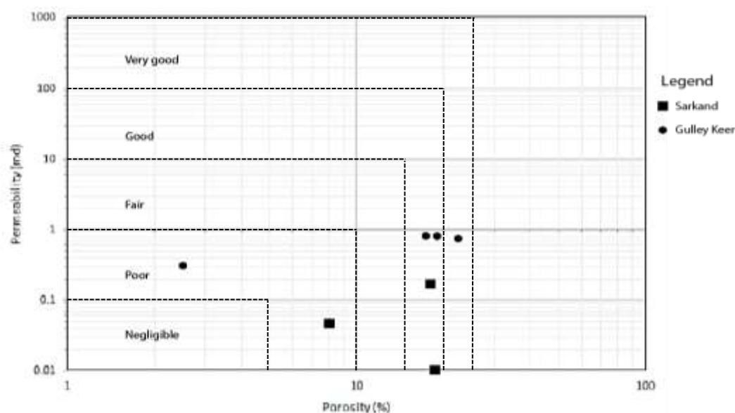
Fig. 7: Cross plot showing porosity vs permeability of Pila Spi samples of the Pila Spi Formation in studied sections. Cross-plot is drawn based on qualitative description of porosity and permeability proposed by [1], [18], and [19].
