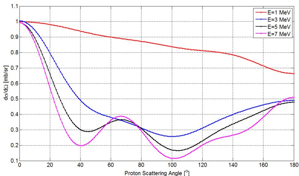
Fig (2): Show the calculated differential cross-sections for the {}^3\text{He}(\text{d},\text{p}){}^4\text{He} reaction as a function of proton scattering angle.
