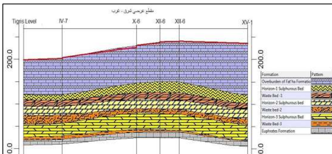
Fig. 3: East-West cross-section of the mineralized beds in the study area
