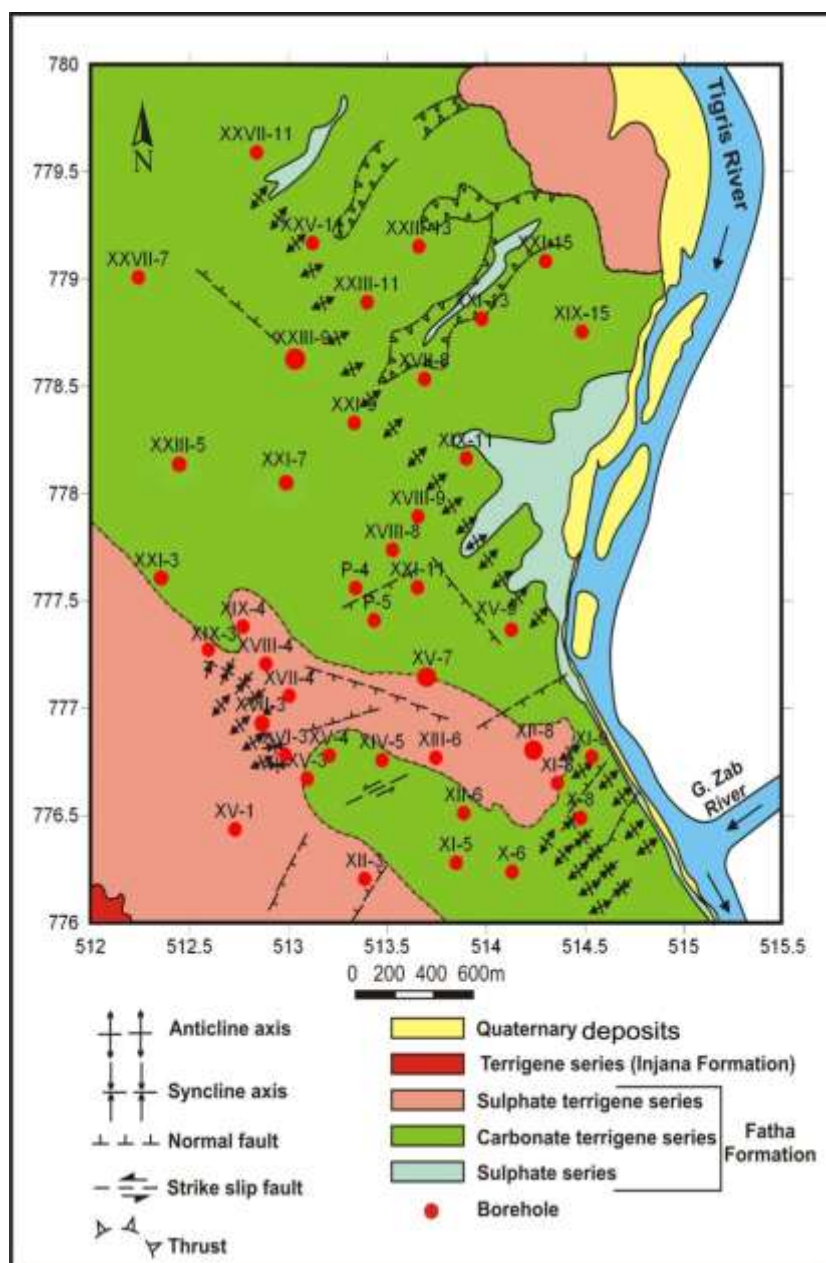
Fig. 1: Geological map of the study area [15]
