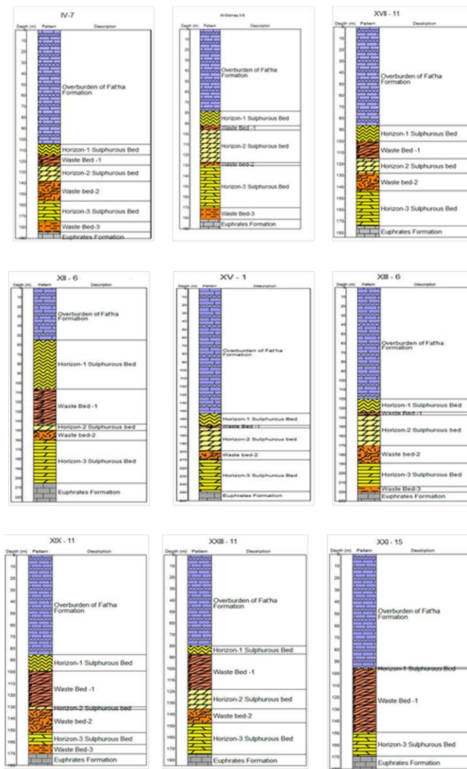
Fig. 2: Sulfur deposits and separating beds
