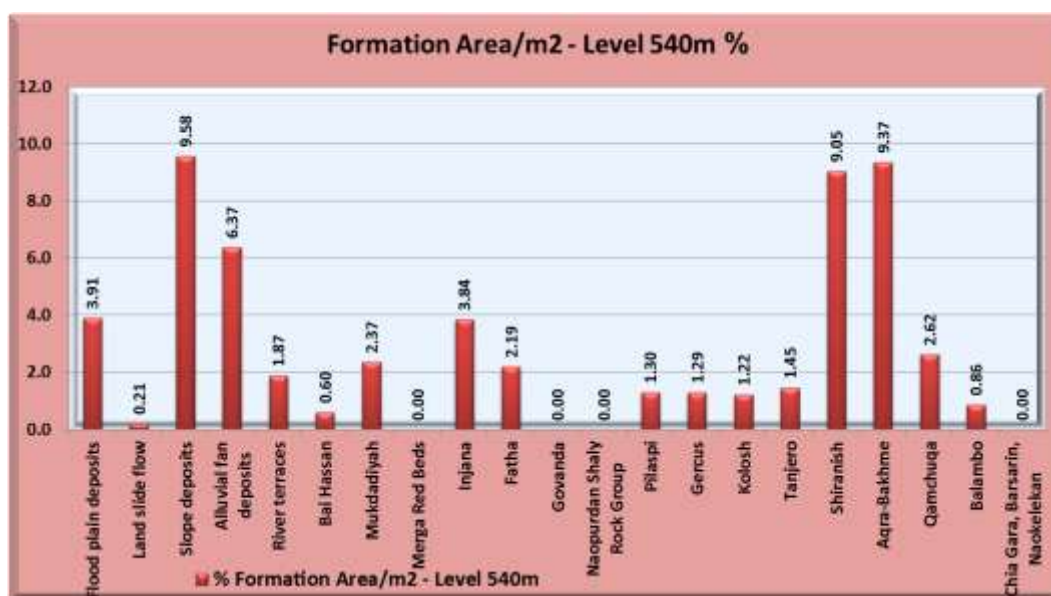
Fig. 22: Diagram showing the% geological immersion area for the level (540) m
