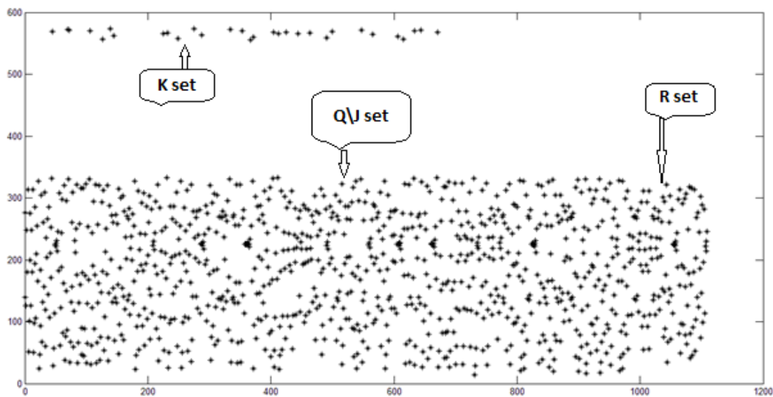
Figure 4 RADG states distribution (case study)
