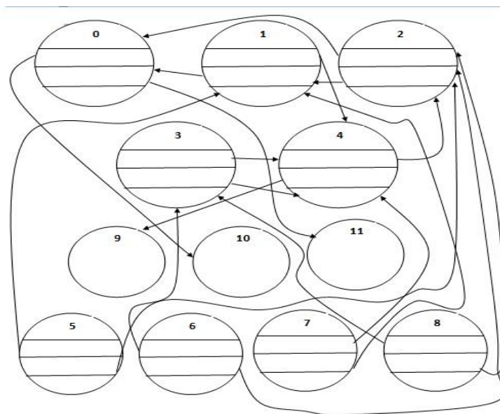
Figure 3 RADG Design Using Auto-Transition Function
