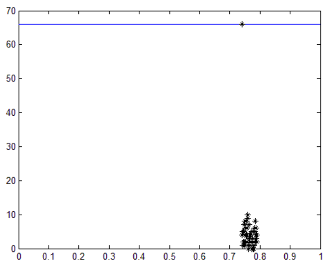
Figure 6 : The comparison RADG design at x_0=0.74 , with 0.741, 0.742, 0.743, ..., 0.79
