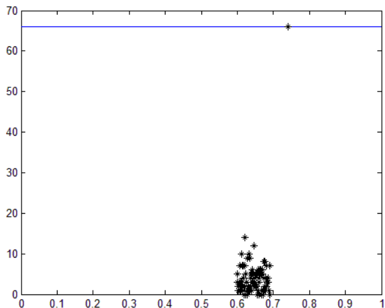
Figure 7 : The comparison RADG design at x_0=0.74 , with 0.6, 0.601, \dots, 0.69
