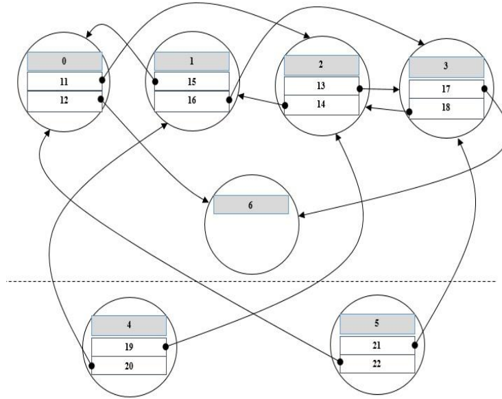
Figure 2 Implementation of RADG algorithm
