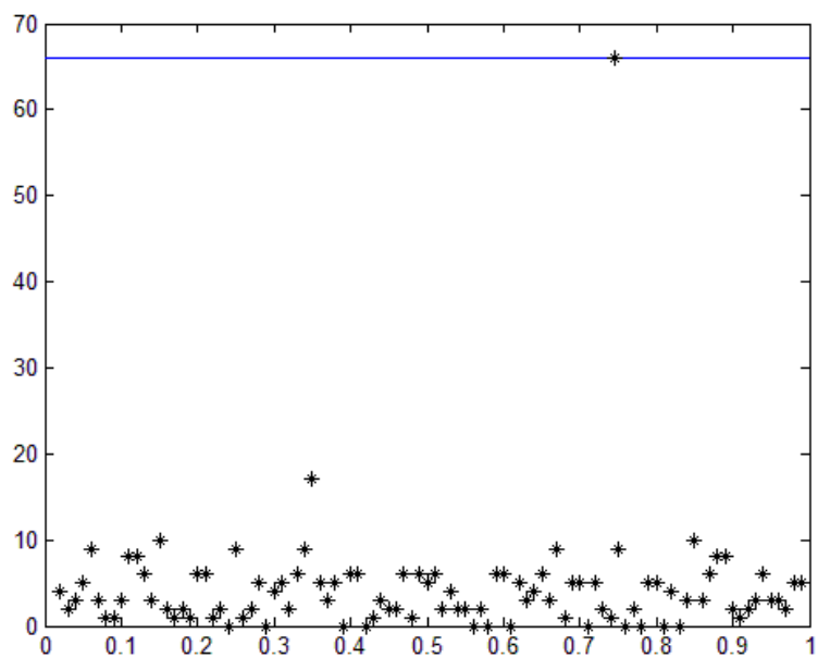
Figure 5 : The comparison RADG design at x_0=0.7459 , with 0.01, 0.02, 0.03, ..., 0.99
