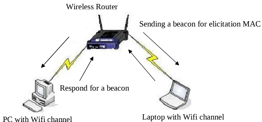
Figure 2: infrastructure network
