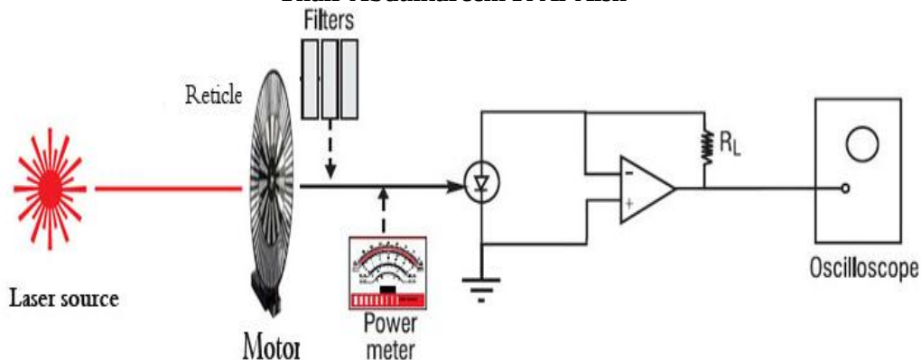
Fig (2): The location of reticle in the optical system
