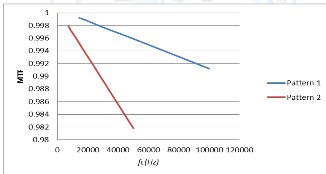
Fig(6) :The relation between MTF versus Chopping frequency f_c
