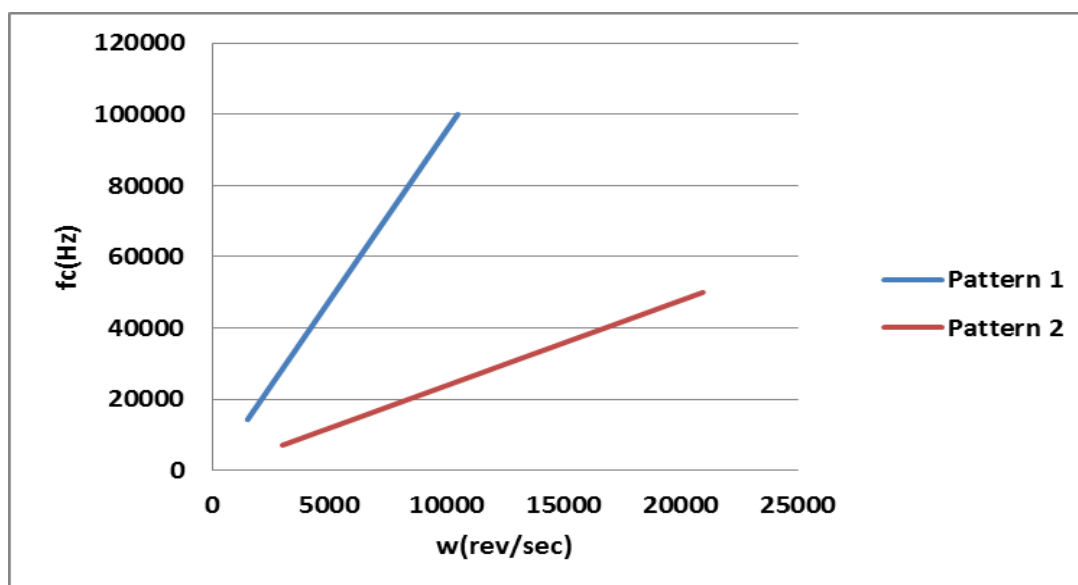
Fig(5) :The relation between Chopping frequency f_c versus angular velocity
