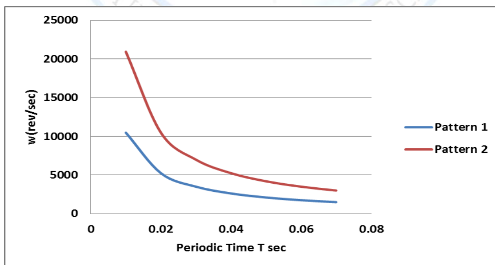
Fig(4) :The relation between angular velocity w versus Periodic Time T (sec)
