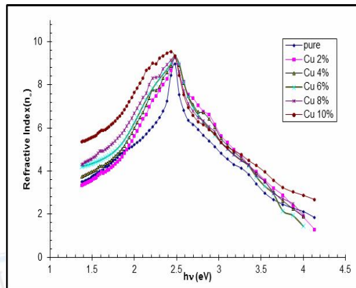
Fig.(7) Refractive index of pure CdS and CdS:Cu films
