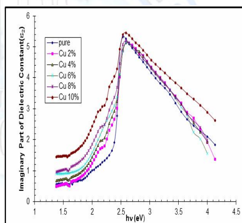
Fig. (9) Imaginary part of dielectric constant of pure CdS and CdS:Cu films
