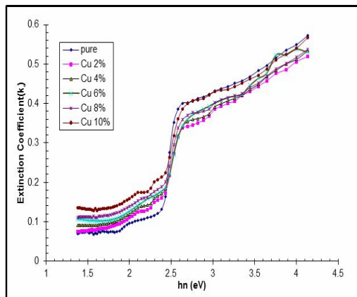
Fig.(6) Extinction coefficient of pure CdS and CdS:Cu films
