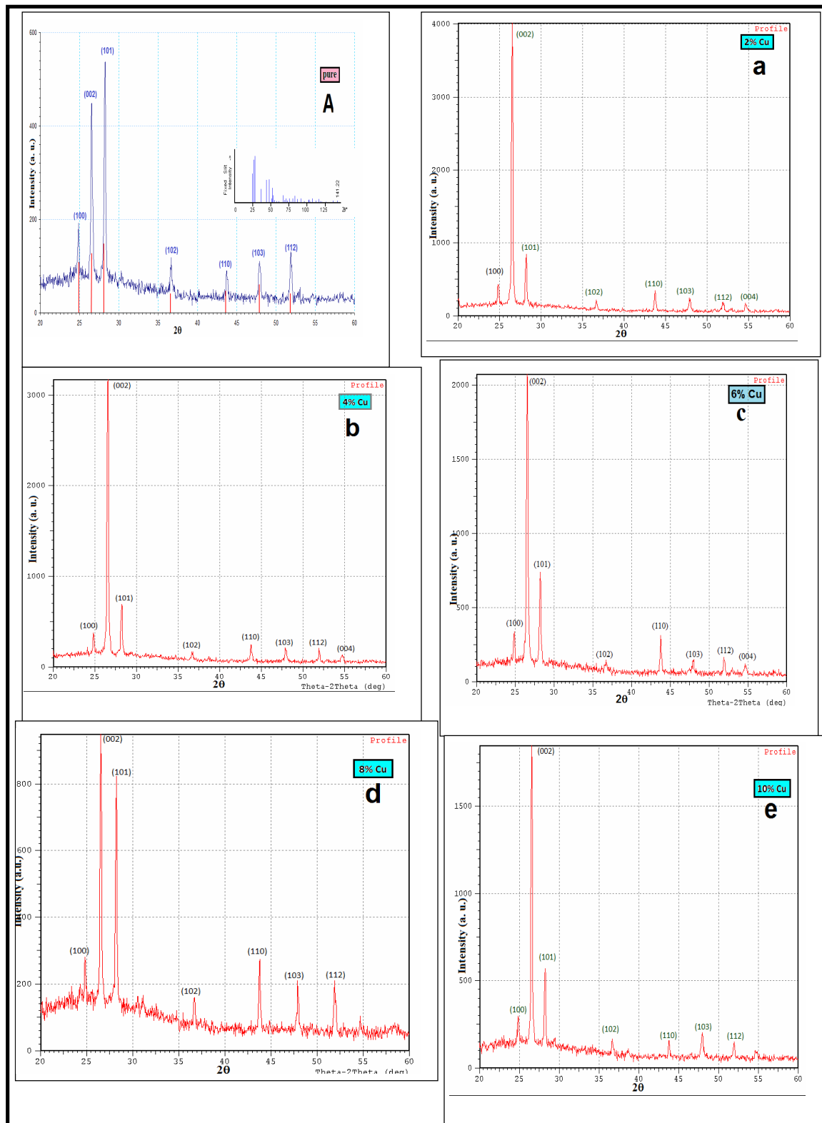
Fig. (1) X-ray diffraction patterns of CdS and CdS:Cu thin films with different concentration
