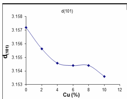
Fig.(2) d_{(101)} as a function of Cu content
