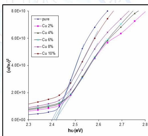
Fig.(5) Relation between (\alpha h\nu)^2 and h\nu for pure CdS and CdS:Cu films
