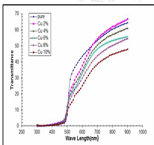
Fig.(4) Transmittance of pure CdS and CdS:Cu films
