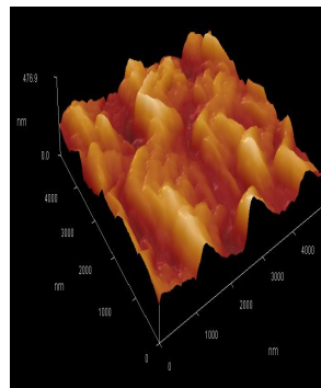
Fig(3) Three-dimensional atomic force microscopy images of films deposited at various Cu concentration
