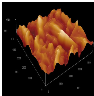
Fig(3) Three-dimensional atomic force microscopy images of films deposited at various Cu concentration
