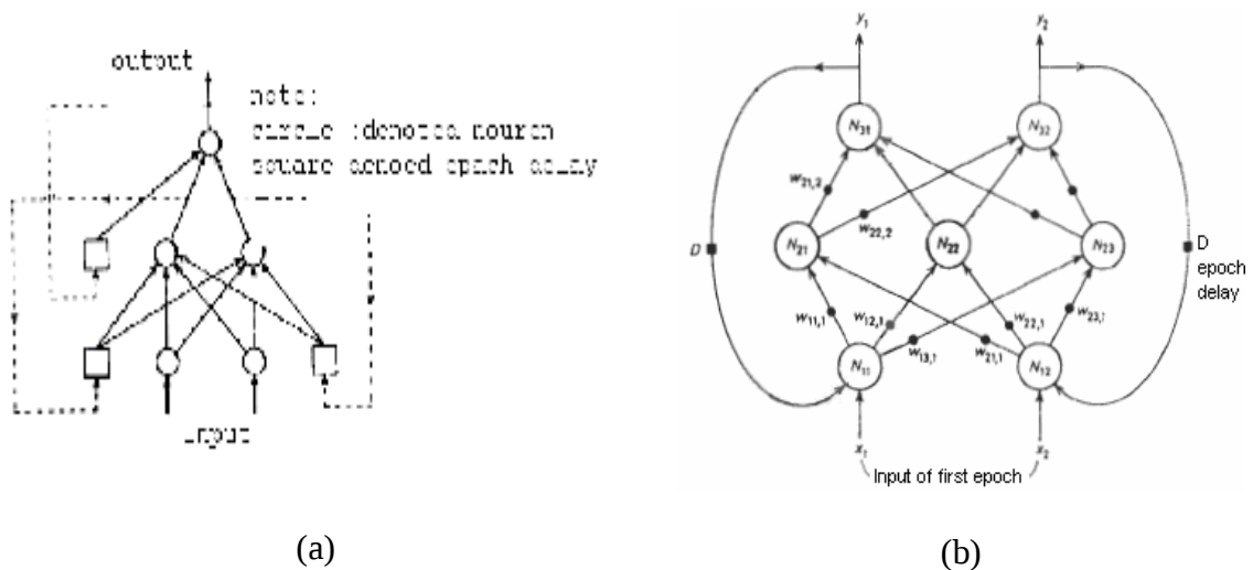
Figure3: a - Fully Recurrent (Time Cycling) Back Propagation ANN b- Recurrent (Time Cycling) Back Propagation ANN
