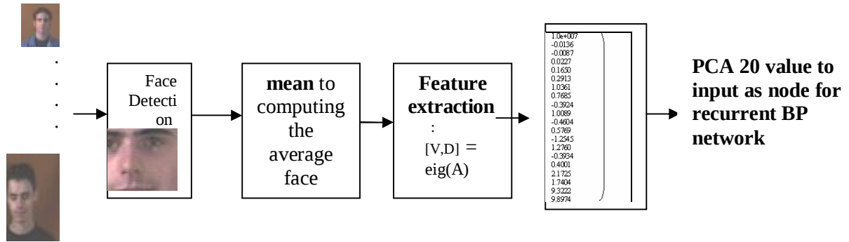
Flow chart for PCA Feature Extraction
