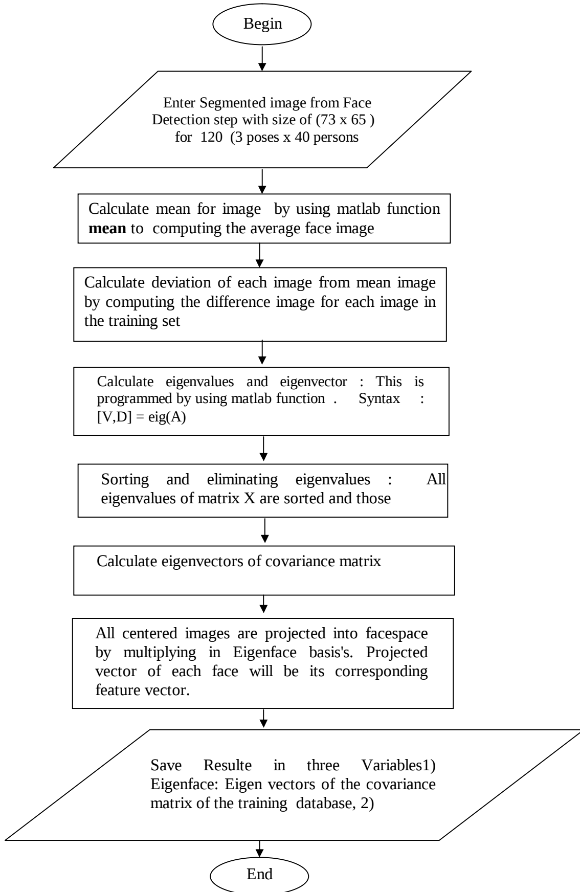
Figure 5: Flow chart for PCA Feature Extraction
