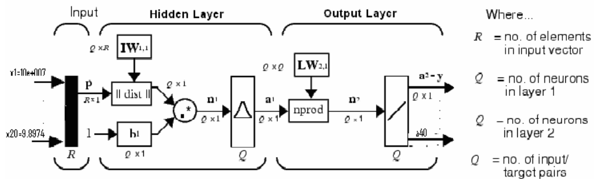
Figure (6) recurrent back propagation neural network
