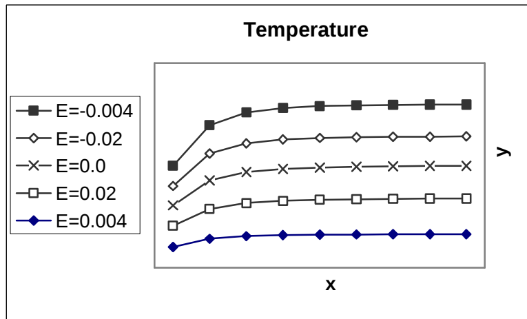
Figure-3: The non-dimensional temperature q on the left side of cavity with different values of dissipation number e
