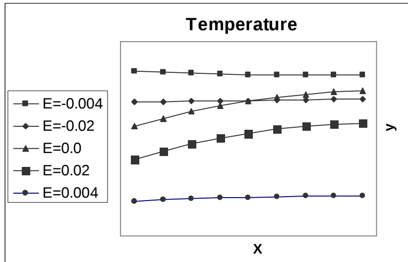
Figure -1: The non-dimensional temperature q on the right side of cavity for different values of dissipation number e
