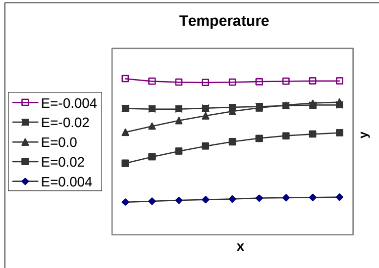
Figure-2: The non-dimensional temperature q in the core of the cavity for different values of dissipation number e
