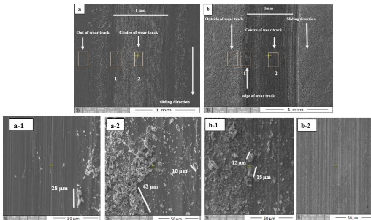
Figure 7: a) SEM image of an overview of steel disc surface without distribution of MoS 2 , a-1) and a-2) enlargements of the worn surface at 1000 X, b) SEM of steel disc surface with the distribution of powders, b-1) and b-2) enlargements of the worn surface at 1000 X.
