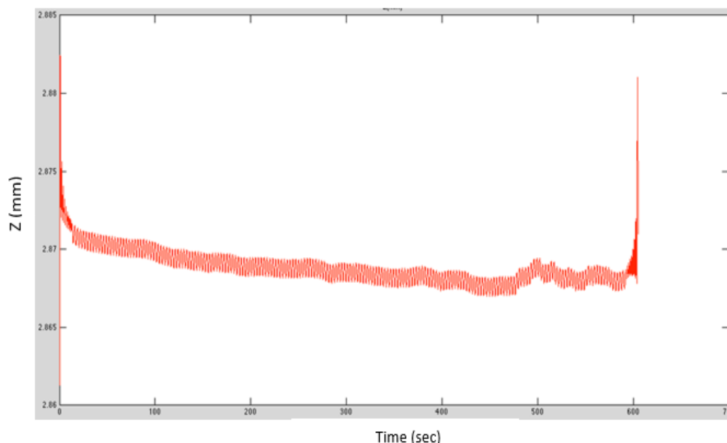
Figure 6: Height location of pin on steel disc with a distribution of particles on the surface ( 3.38 \times 10^{17} per \text{m}^2 ). With time (10 min), normal load (0.5 kg), revolution of the disc (20 rpm), and wear track on the surface (25mm)
