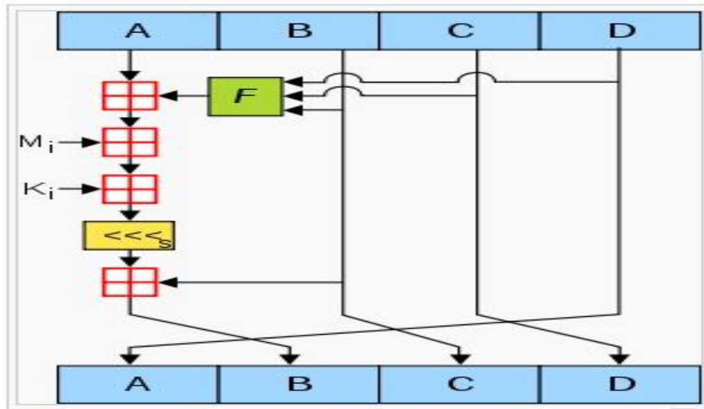
fig 1 : md5 operation within a round
