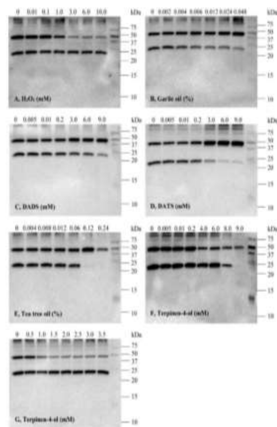
Figure 2. The effects of treating Jurkat T-lymphocytes with H 2 O 2 , garlic oil, DADS, DATS, tea tree oil or terpinen-4-ol on the redox/oligomerization state of the typical 2-Cys Prx proteins. Gels identical to those shown in Figure 1 were run and the proteins thus separated were subjected to immunoblot analysis using the anti-(typical 2-Cys Prx) antibodies (see antibody details).
