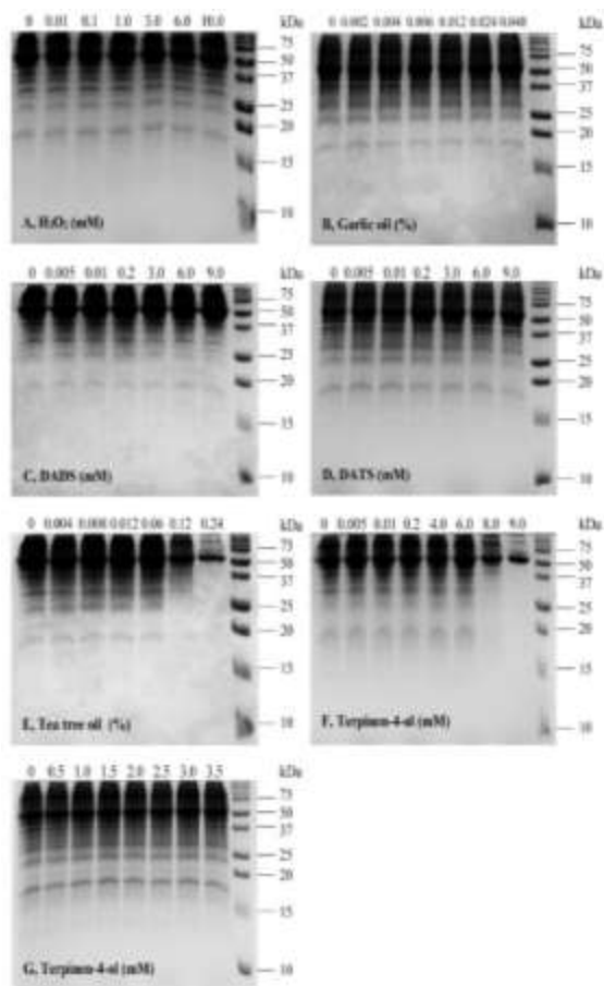
Figure 1. The effects of treating Jurkat T-lymphocytes with H 2 O 2 , garlic oil, DADS, DATS, tea tree oil or terpinen-4-ol on the total soluble proteins extracted from the cells. The proteins (30 µg protein per well) were separated using NR-PAGE and then stained using Coomassie Blue.
