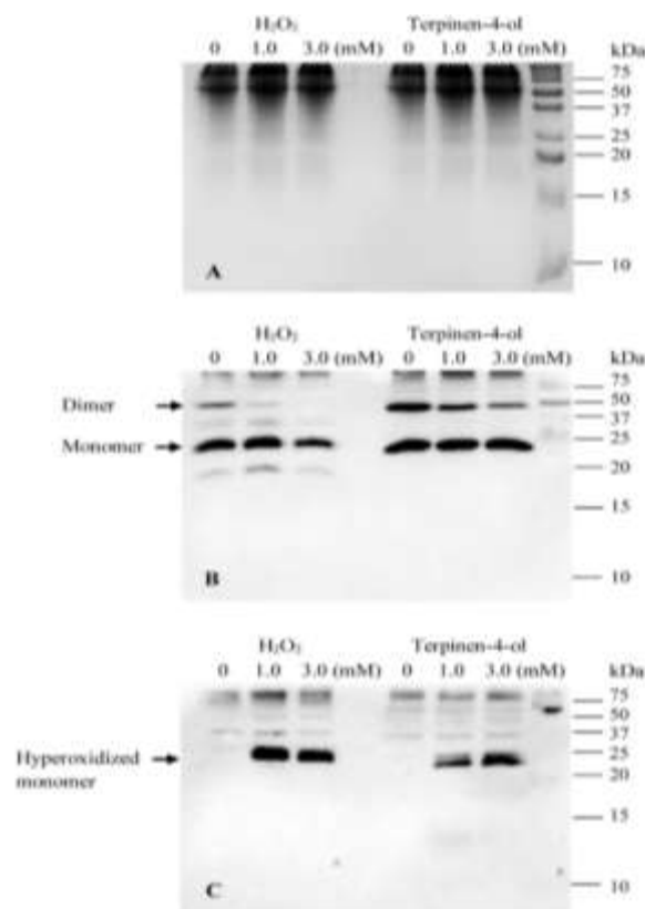
Figure 3. The effects of treating Jurkat T-lymphocytes with H_2O_2 or terpinen-4-ol on the redox/oligomerization state of the typical 2-Cys Prx proteins. The total soluble proteins were extracted from the cells and separated using NR-PAGE. In panel A, the proteins were stained using Coomassie Blue. In panel B, the proteins were subjected to immunoblot analysis using the same antibodies as described in the caption to Figure 2. In panel C, the hyperoxidised form of the typical 2-Cys Prx proteins was detected using commercially available anti-(Prx-SO 3 ) antibodies (see antibody details).
