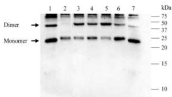
Figure 4. The effects of treating Jurkat T-lymphocytes with H_2O_2 , garlic oil, DADS, DATS, tea tree oil or terpinen-4-ol on the redox/oligomerization state of Prx1. The total soluble proteins were extracted from the cells and then separated using NR-PAGE. Prx1 was detected using antibodies raised against the peptide PLVSDPKRTIAQDY which is unique to human Prx1. Lane 1 contains the extract from the control cells. Lanes 2 through 7 contain extracts from cells treated with 3 mM H_2O_2 (Lane 2), 0.048% (v/v) garlic oil (Lane 3), 3 mM DADS (Lane 4), 3 mM DATS (Lane 5), 0.06% (v/v) tea tree oil (Lane 6) and 3 mM terpinen-4-ol (Lane 7).
