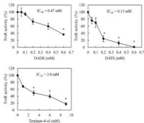
Figure 5. The effects of DADS, DATS and terpinen-4-ol on TrxR enzyme activity in crude extracts from Jurkat T-lymphocytes. The data are expressed as % of the untreated control and each data point is the mean value for 3 replicate wells. The vertical bars represent \pm standard error of the mean ( n = 3 ). A star indicates a significant difference from the untreated control ( p < 0.05 ).
