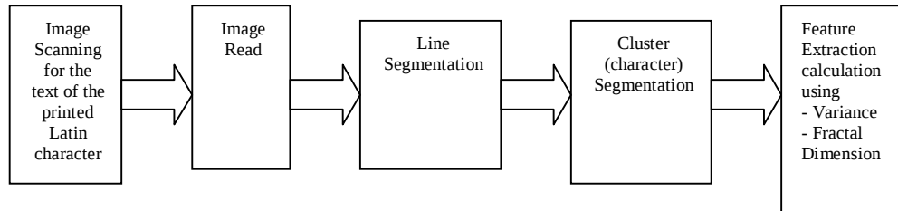
Figure 4: Feature Extraction Building file
