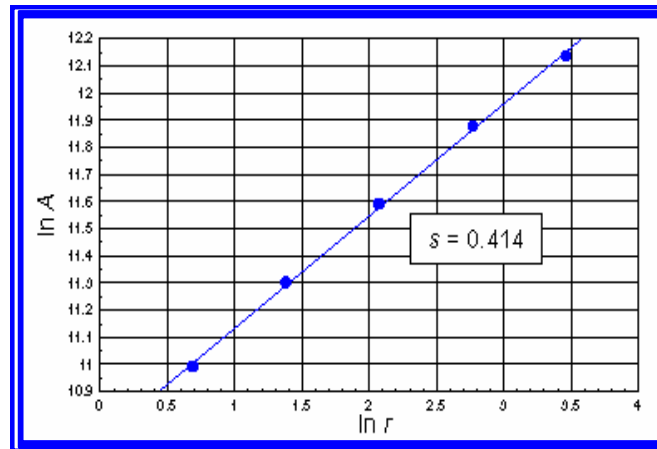
Figure 6: Richardson-Mandelbrot plot for the area of a binary structure at different box sizes (in pixels)
