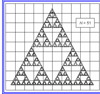
Figure 5: Sierpinsky gasket overlaid with a grid of squares
