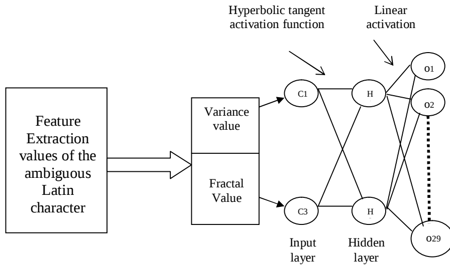
Figure 8: Back Propagation Neural Network of 2-2-29 (testing phase)
