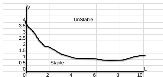
Fig. (1-4): show the stability areas the diffusion equation (14) when D= 0.2 , 0.4 , 0.6
