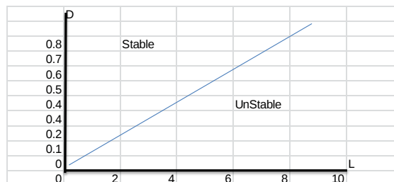
Fig. (1-3): show the stability areas the load equation (12) when V= 0.2 , 0.4 , 0.6
