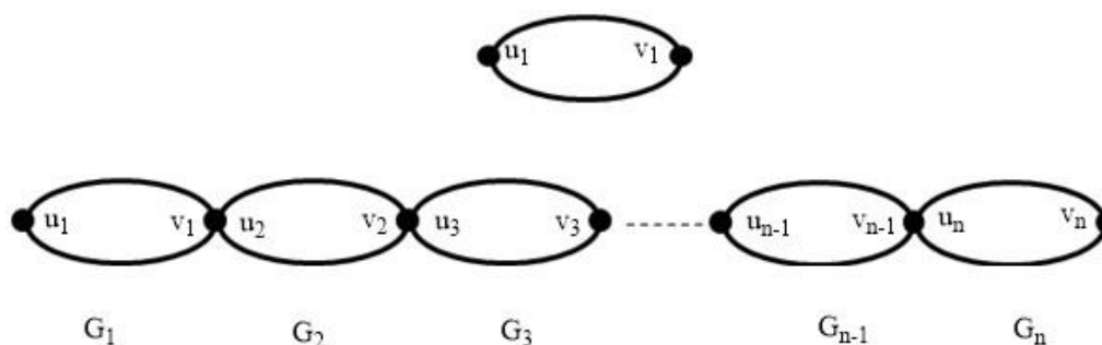
Fig. 3-1. Chain fuzzy graphs
