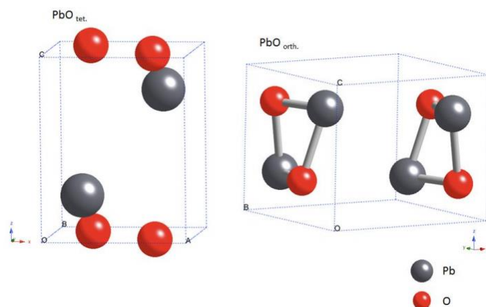
Fig. 1 A diagram displaying the PbO crystal structure [15]
