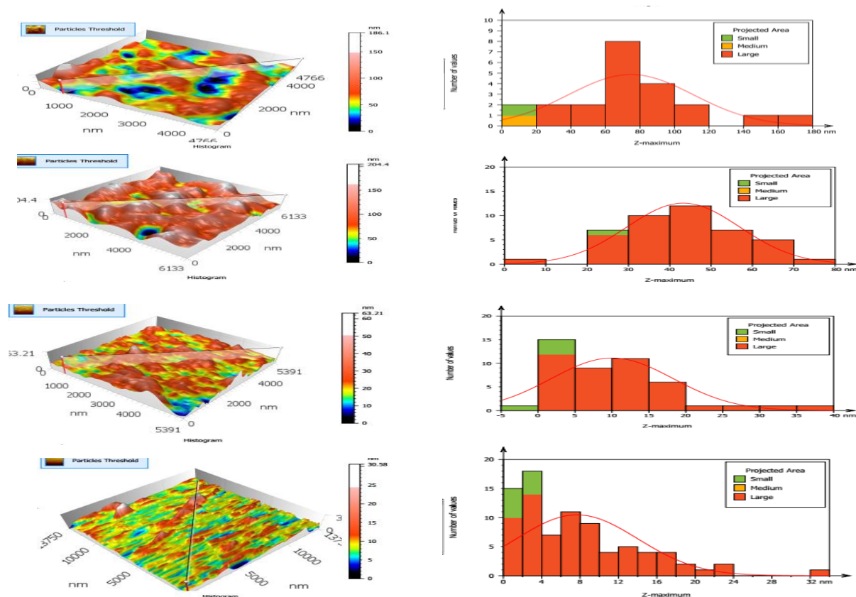
Figure.3 PbO's structural characteristics at different bombardment times (4, 6, 8, and 10 minutes).
