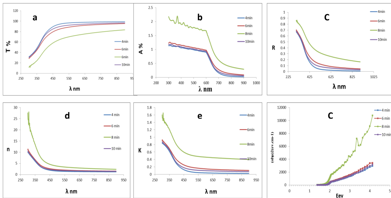
Figure.6 period of the bombardment's impact on the optical characteristics a. transition b. absorption c. reflective d. refractive index e. extinction coefficient f. energy gap.
