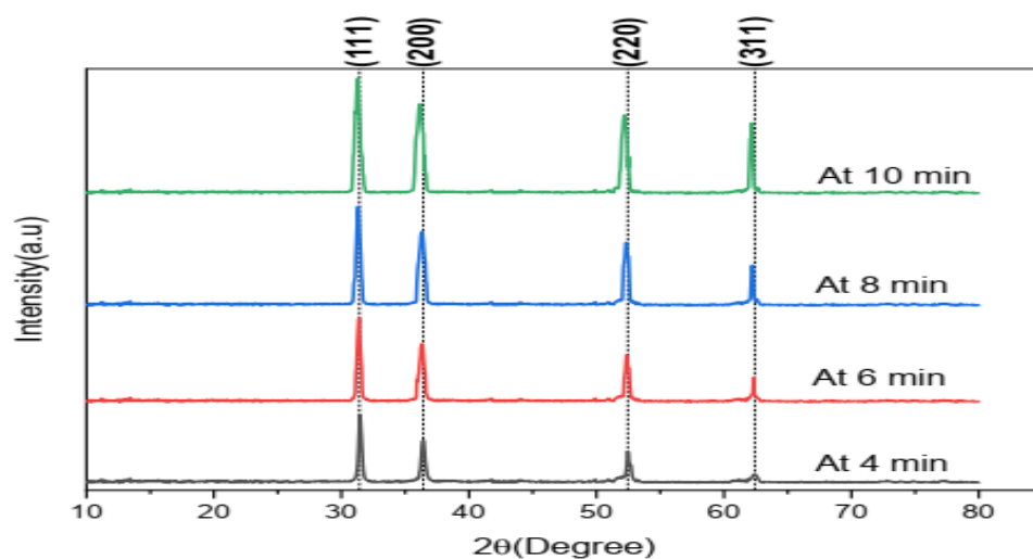
Figure 4 displays the induced plasma bombardment-induced X-ray diffraction of PbO metal oxide after various times of preparation.
