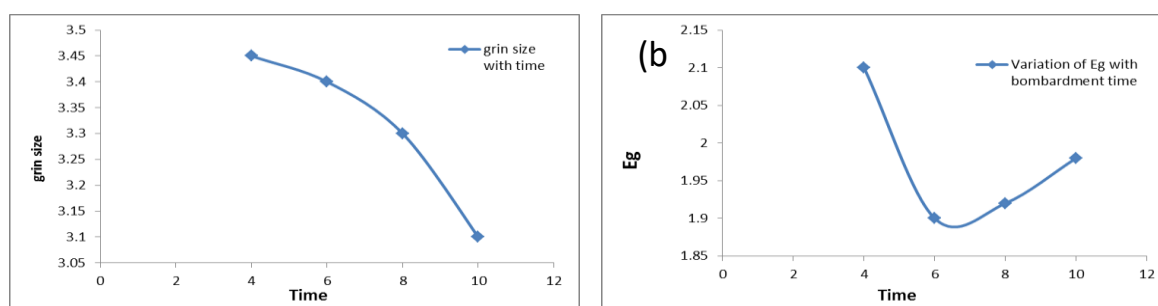
Figure. 2-a- Variation of grain size with bombardment time, b- Variation of E_g with bombardment time
