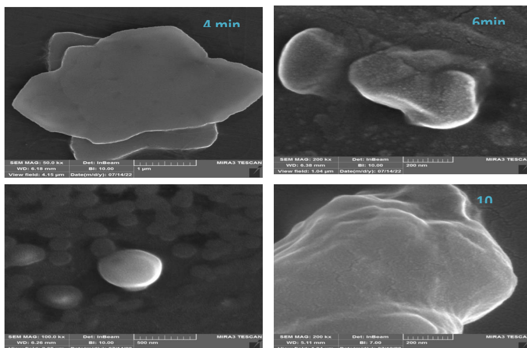
Figure (5) SEM images of PbO prepared at different bombardment periods (4,6,8,10 min).
