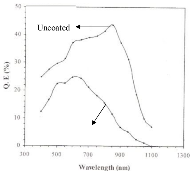
Figure 5. Quantum Efficiency of Si Photodetector before and after Pt deposition .
