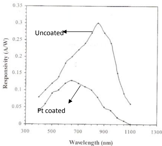
Figure 4. Spectral Responsivity of Si Photodetector before and after Pt deposition .
