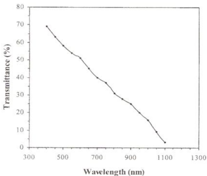
Figure 2. Spectral Transmittance of Pt Thin Film
