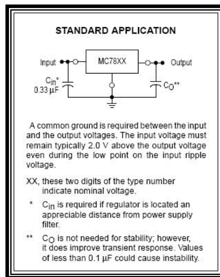
Figure (5-b): 7805 Typical application
