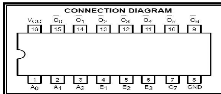
Figure (4): 74LS138 Pin assignment
