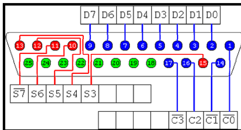
Figure (1) 25-way Female D-Type Connector
