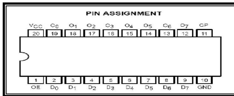
Figure (3): 74LS574 Pin assignment
