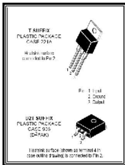
Figure (5-a): 7805 Pin assignment
