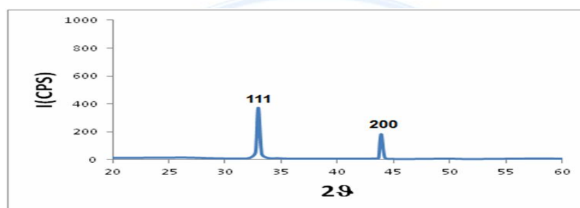
Figure (4): XRD diagram of silver thin film
