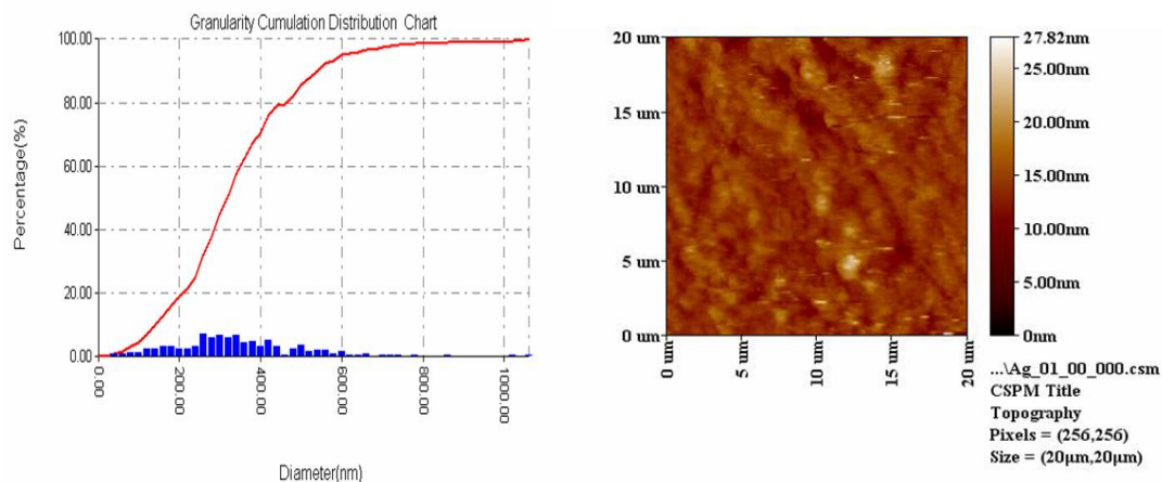
Figure (2). AFM image of Ag particle
