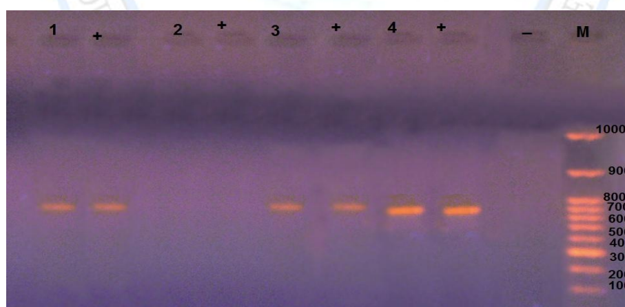
Figure 1: Amplified product of the DNA from samples detected by various method Lanes 1-4 amplified product of DNA extracted by method 1-4 respectively, lane (+) control positive to each method and M 100bp marker.
