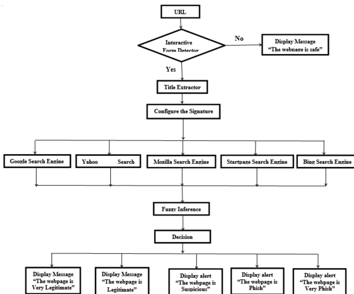
Figure 2: Flowchart of Proposed Algorithm
