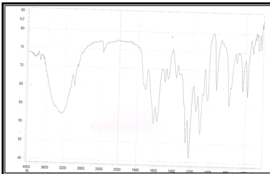
Fig. (1) : FT-IR. Spectrum of (L) ligand ( C_{19}H_{16}N_4O_2 )
