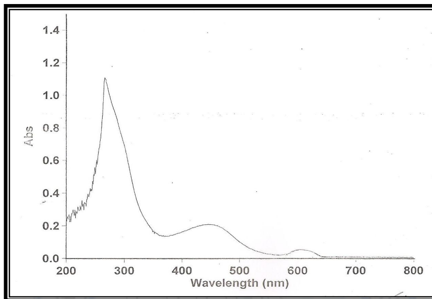
Fig. (4) : UV-Visible Spectrum of Ni (II) Complex
