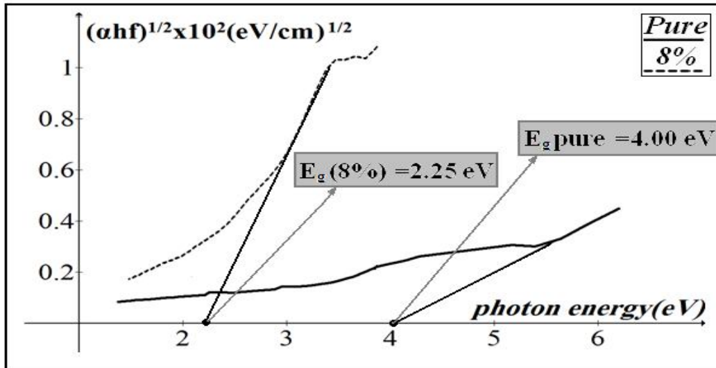
Fig. (3) Optical energy band gap of pure PVA , 8 wt%, KMnO 4 doped PVA samples.
