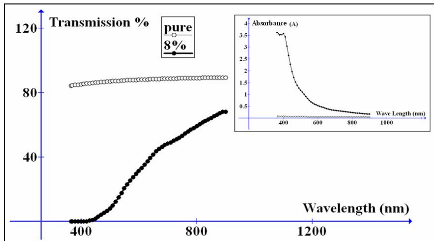
Figure (1) Transmittance against Wavelength for pure PVA , 8wt% KMnO 4 doped PVA samples. The inset shows the Absorbance vs. Wavelength.
