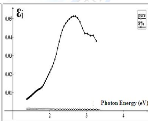
Fig. (5) \epsilon_i vs. Photon energy.
