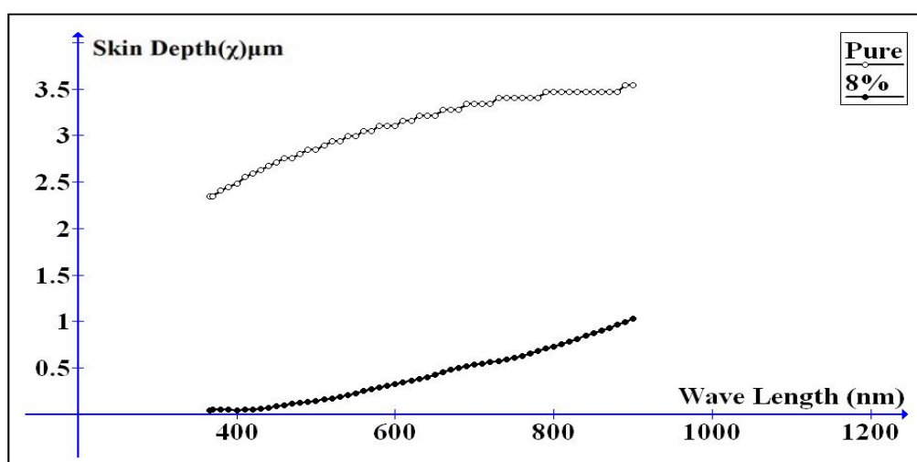
Fig. (7) Skin depth ( \chi ) as a function of wavelength.
