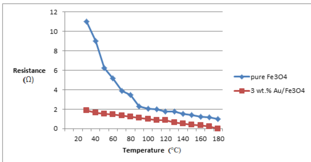
Figure 5: Relationship of resistance against temperature of pure \text{Fe}_3\text{O}_4 and 3 wt.% Au/ \text{Fe}_3\text{O}_4
