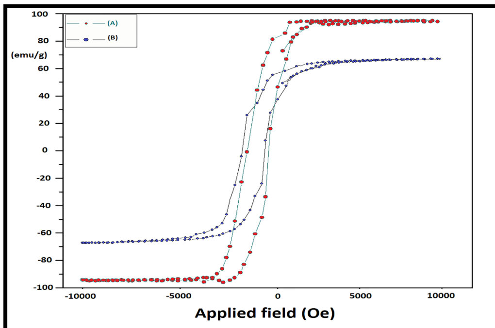
Figure 6: M against applied field plot of (a) pure \text{Fe}_3\text{O}_4 , and (b) 3 wt.% \text{Au}/\text{Fe}_3\text{O}_4
