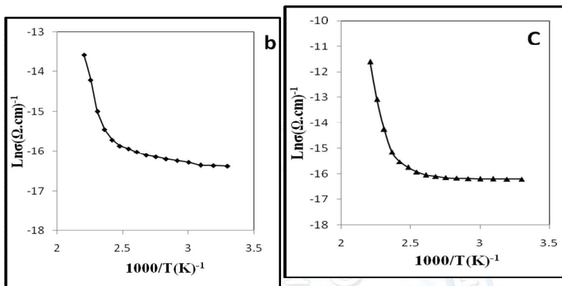
Figure (11): ( \ln \sigma ) versus ( 1000/T ) of BaTiO 3 films at as deposited ( T_s=573K ) and different doping ; ( a) MoO 3 , (b) V 2 O 5 , (c) NiO.
