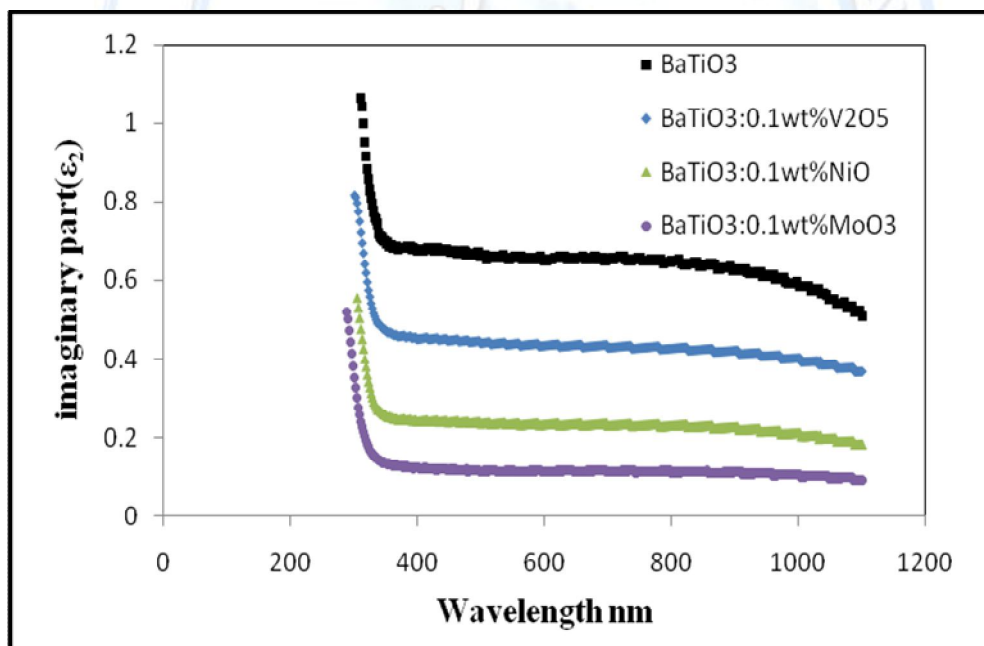
Figure (14): the variation of the imaginary part ( \epsilon_i ) with wavelength of the BaTiO 3 films at different doping (MoO 3 , V 2 O 5 and NiO) at substrate temperature (573K).
