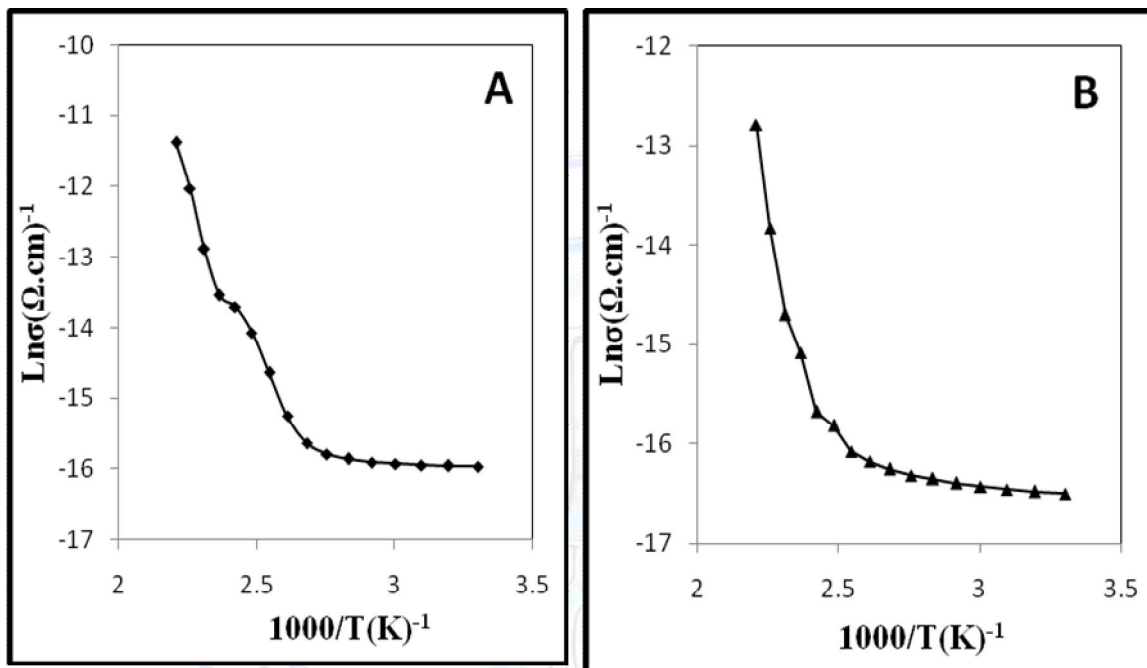
Figure (16): ( \ln \sigma ) versus ( 1000/T ) of BaTiO 3 films at different annealed temperatures (A) 673K (B) 773K.
