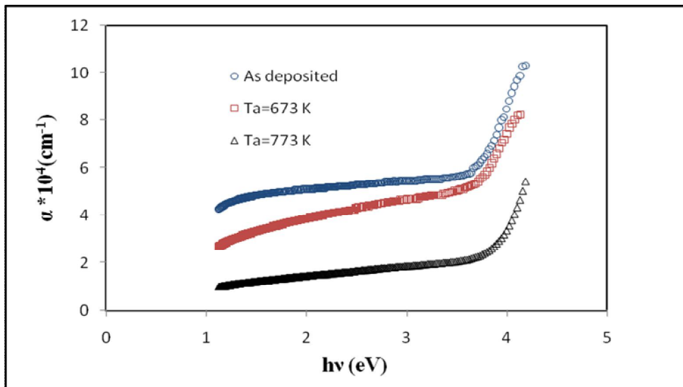
Figure (3): the variation of the absorption coefficient ( \alpha ) with photon energy of the BaTiO 3 films for as deposited ( T_s=573K ) and annealed at (673K, 773K).
