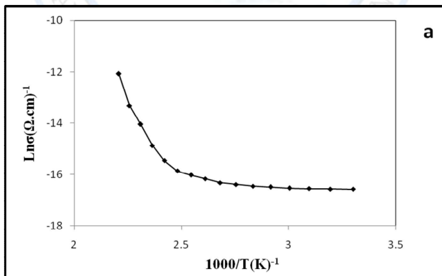
Figure (16): ( \ln \sigma ) versus ( 1000/T ) of BaTiO 3 films at different annealed temperatures (A) 673K (B) 773K.
