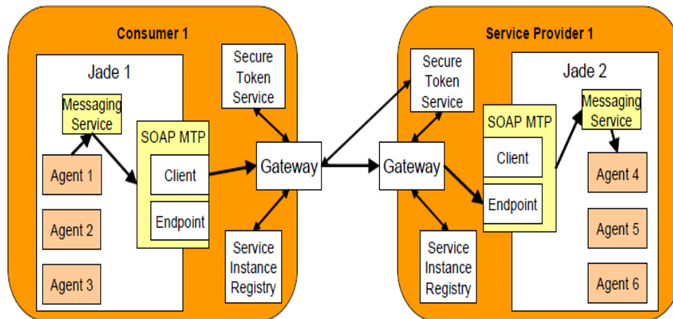
Figure 2: Enterprise Agent Interoperable Schema
