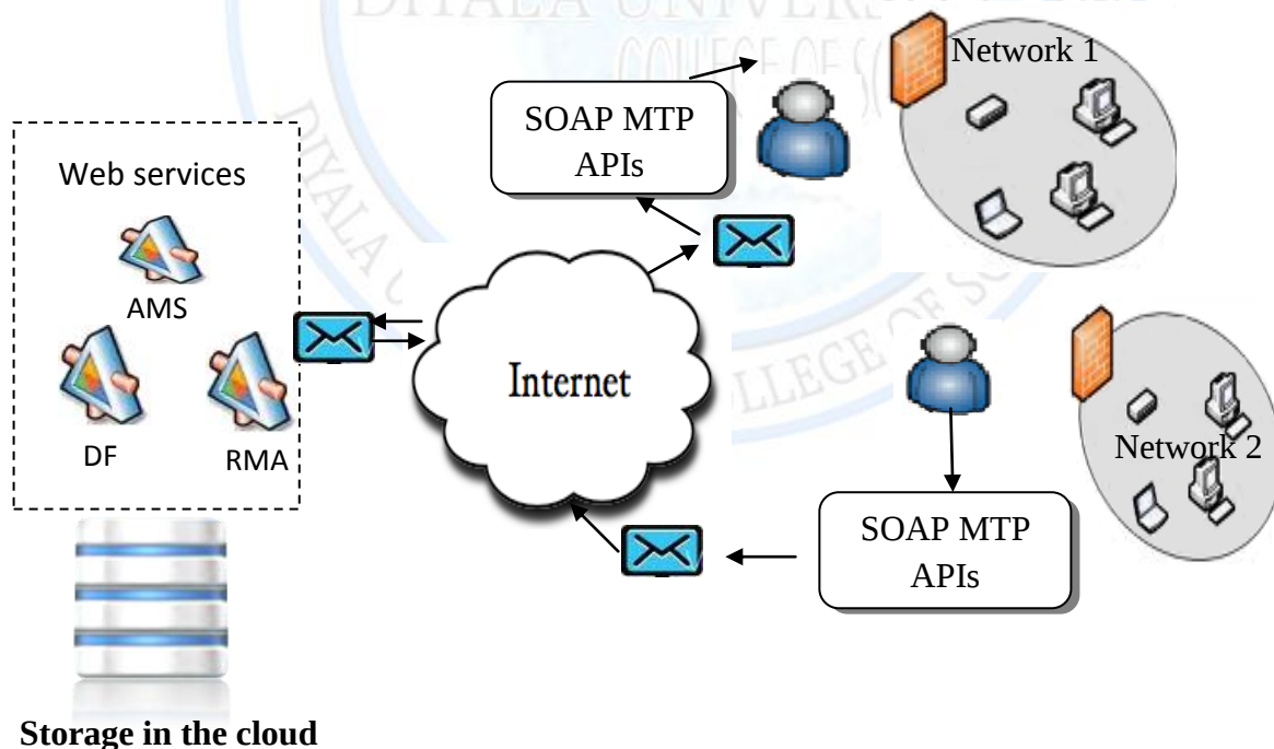
Figure 5: Web Based Firewall Agent Communication Schema
