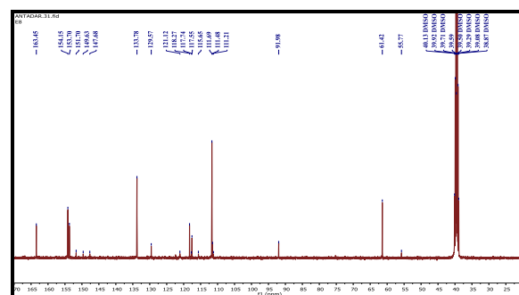
Fig 12: ^{13}\text{C} -NMR spectrum of compound 4-(4-(dimethylamino)phenyl)-6-(4-hydroxy-3-methoxyphenyl)-2-oxo-1,2-dihydropyridine-3-carbonitrile
