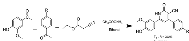
Scheme1. Synthesis of 1-(4-hydroxy-3-methoxyphenyl) ethan-1-one derivatives T 1 – T 3
