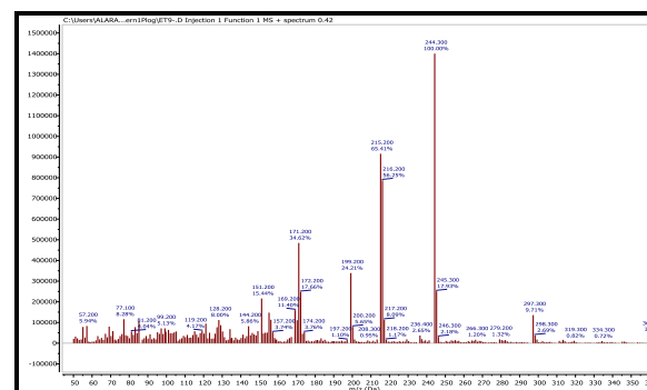
Fig 13: mass spectrum of compound 4-(4-(dimethylamino)phenyl)-6-(4-hydroxy-3-methoxyphenyl)-2-oxo-1,2-dihydropyridine-3-carbonitrile
