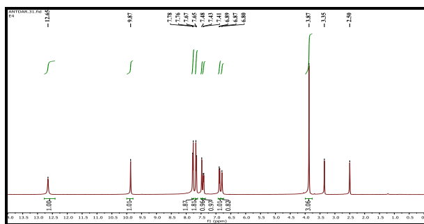
Fig 7: ^1\text{H} -NMR spectrum of compound 4-(4-bromophenyl)-6-(4-hydroxy-3-methoxyphenyl)-2-oxo-1,2-dihydropyridine-3-carbonitrile
