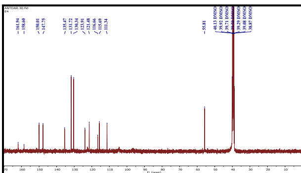
Fig 8: ^{13}\text{C} -NMR spectrum of compound 4-(4-bromophenyl)-6-(4-hydroxy-3-methoxyphenyl)-2-oxo-1,2-dihydropyridine-3-carbonitrile
