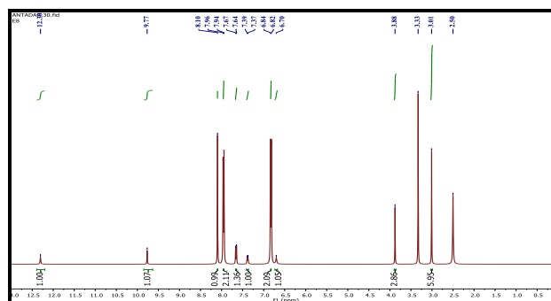
Fig 11: ^1\text{H} -NMR spectrum of compound 4-(4-(dimethylamino)phenyl)-6-(4-hydroxy-3-methoxyphenyl)-2-oxo-1,2-dihydropyridine-3-carbonitrile
