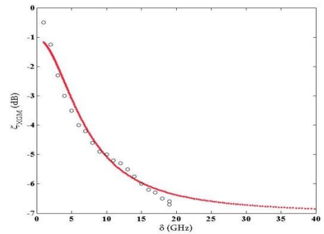
Fig. 5. XGM conversion efficiency at 0.2mW pump power and different powers of probe pulse.
