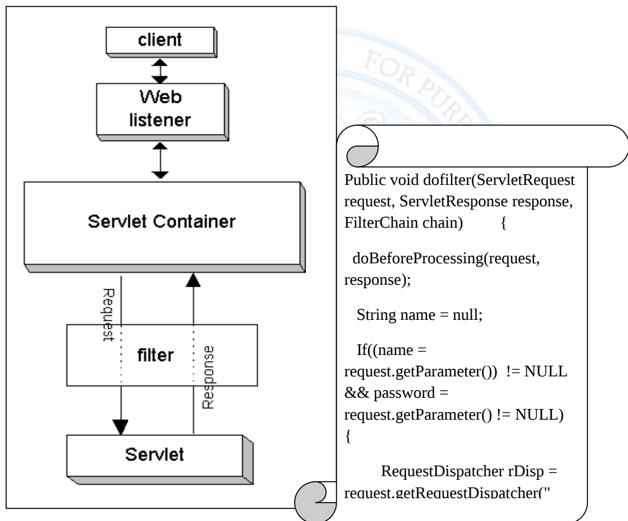
Figure (8): Servlet Filter installed to Capture HTTP packet and forward it to other Processing Elements
