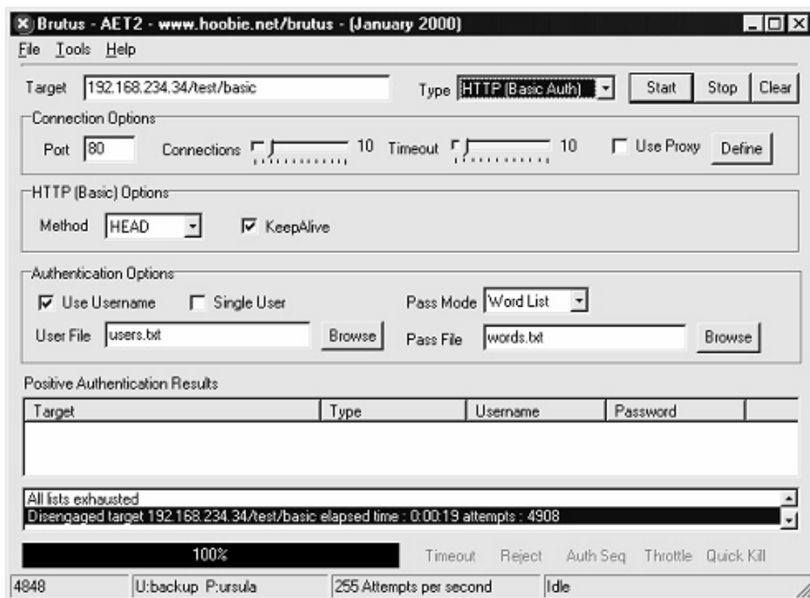
Figure (3): the main page of the Brutus application
