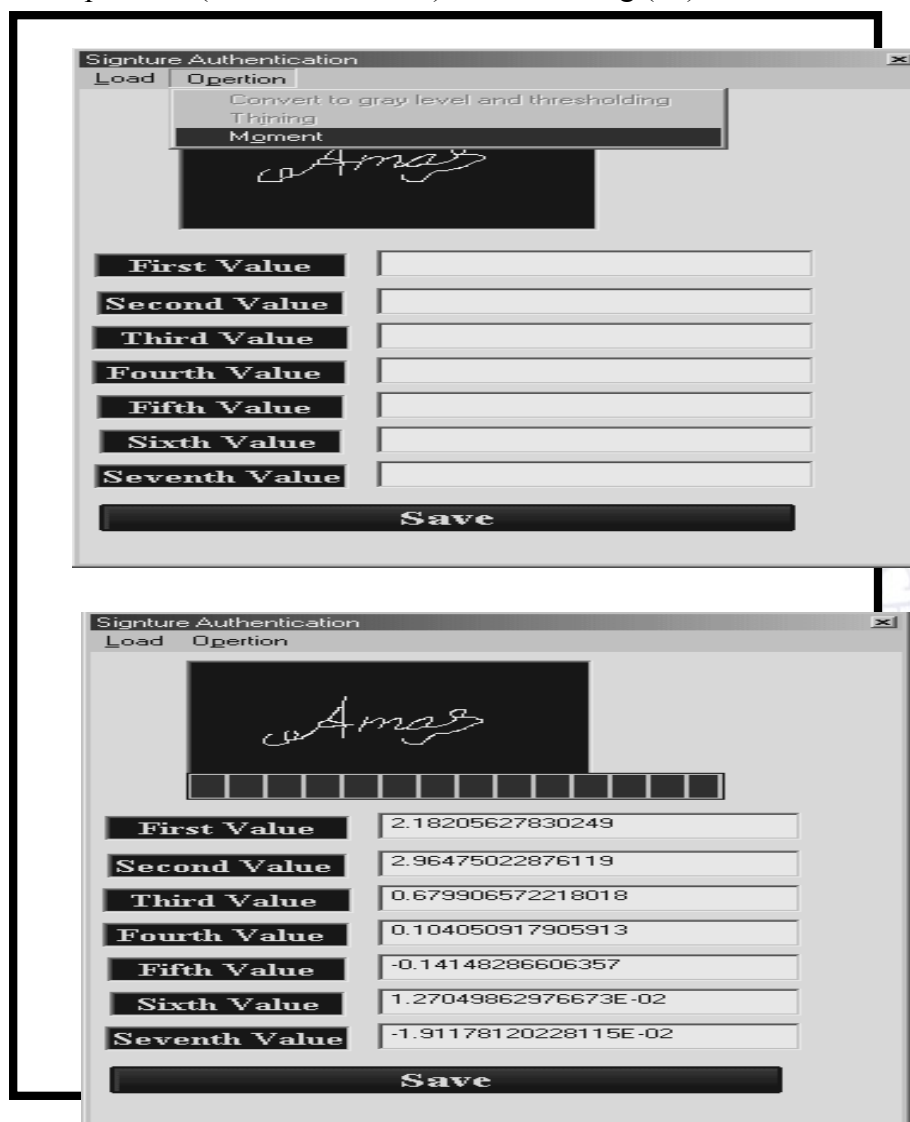
Fig.(10) The Moment Operation (feature extraction)
