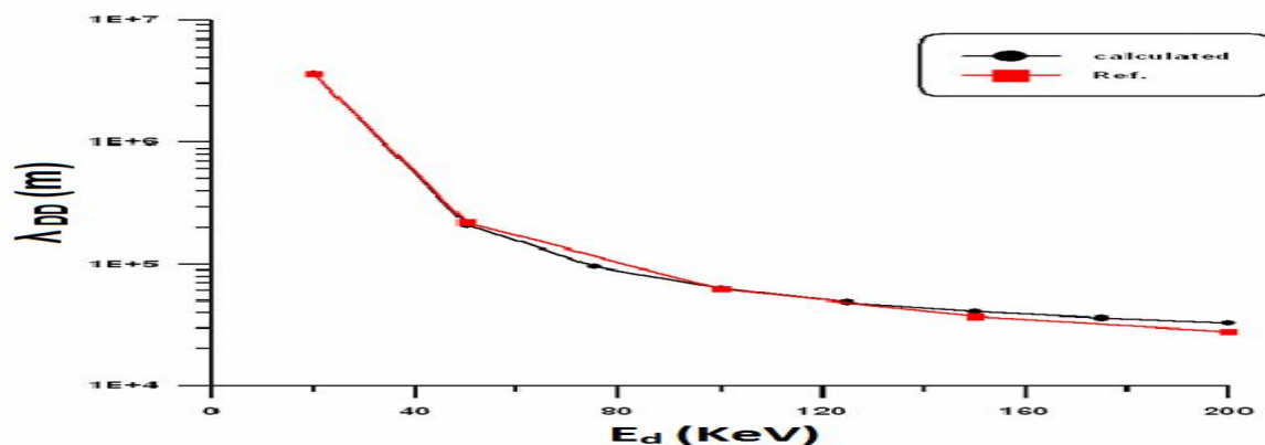
Fig.(5): Mean free path for D-D reaction versus incident deuteron energy for n_i=10^{25} \text{ m}^{-3} after correction.
