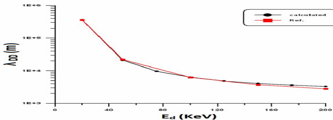
Fig.(6): Mean free path for D-D reaction versus incident deuteron energy for n_i=10^{26} \text{ m}^{-3} after correction.
