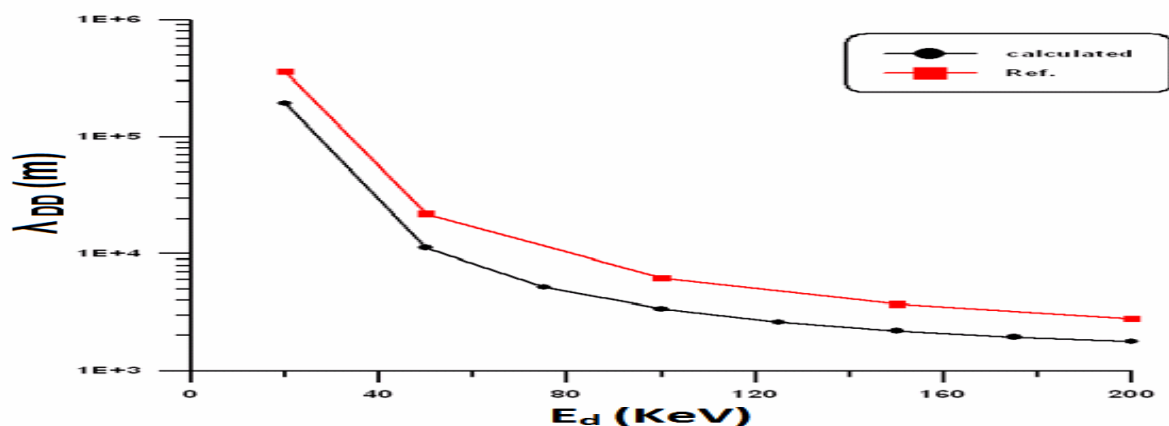
Fig.(3): Mean free path for D-D reaction versus incident deuteron energy for n_i=10^{26} \text{ m}^{-3} before correction.
