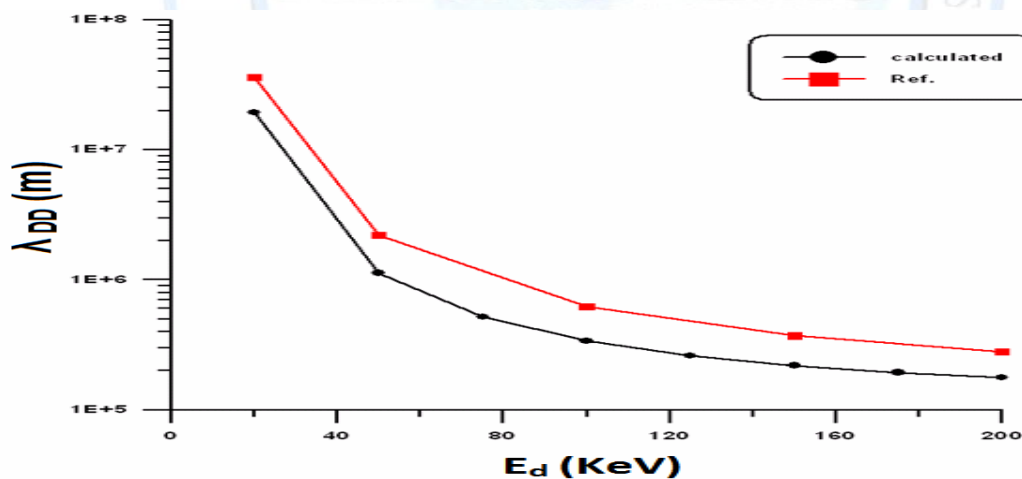
Fig.(2): Mean free path for D-D reaction versus incident deuteron energy for n_i = 10^{25} \text{ m}^{-3} before correction.
