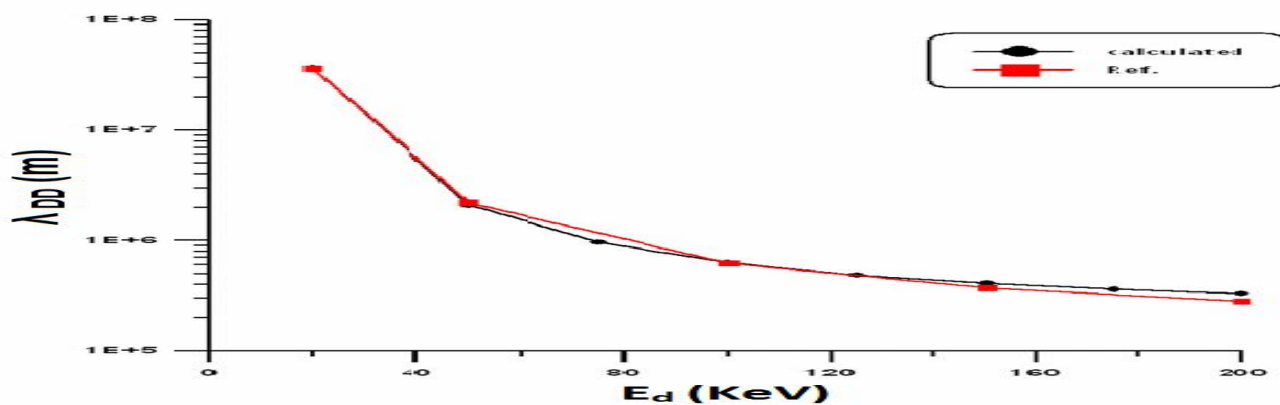
Fig.(4) : Mean free path for D-D reaction versus incident deuteron energy for n_i=10^{24} \text{ m}^{-3} after correction.
