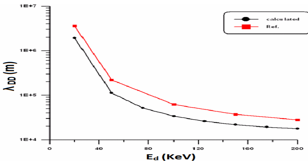
Mean free path for D-D reaction versus incident deuteron energy for n_i = 10^{24} \text{ m}^{-3} before correction. Fig.(1):
