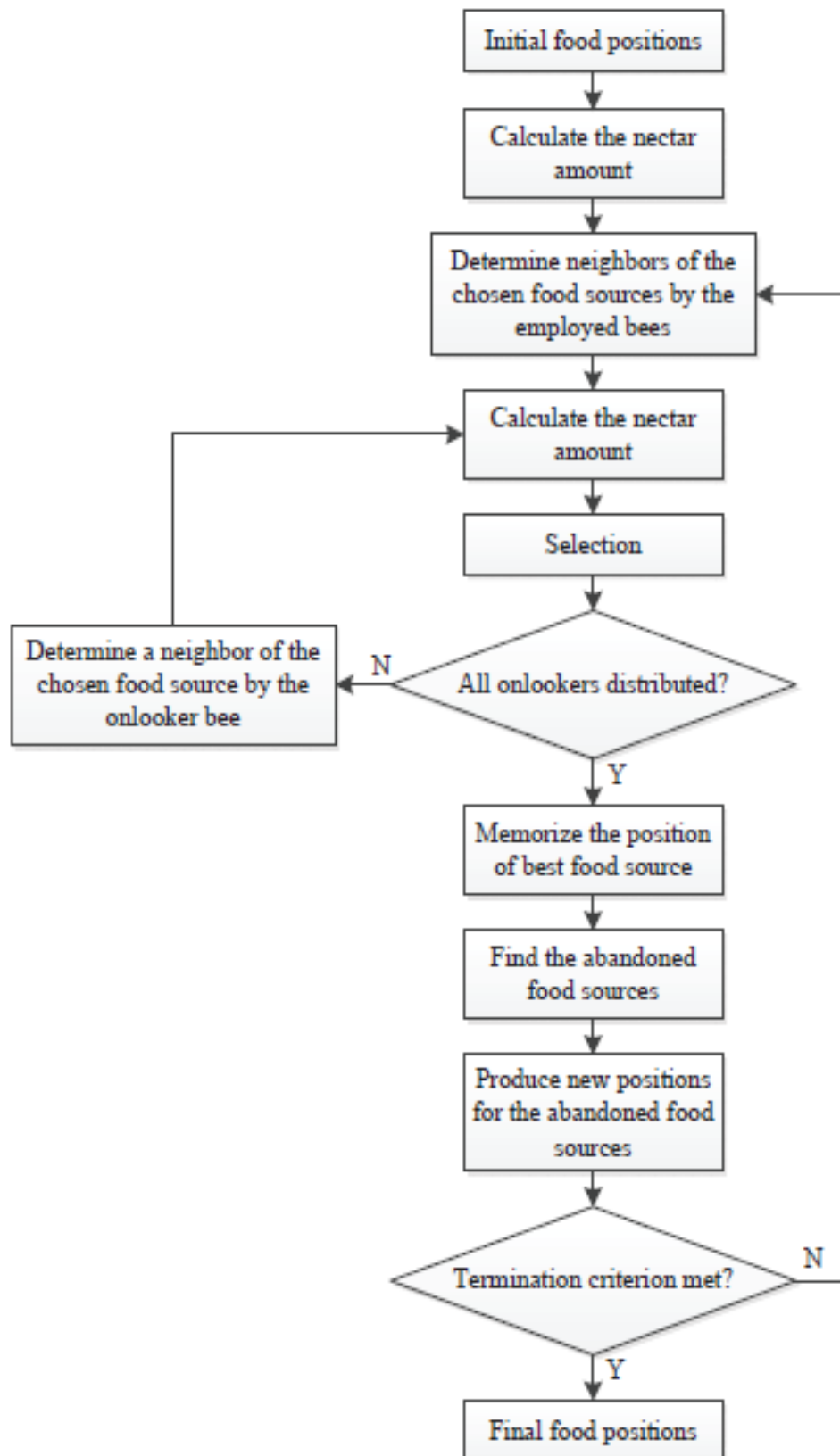
Fig.(1) Flow Chart of ABC Algorithm
