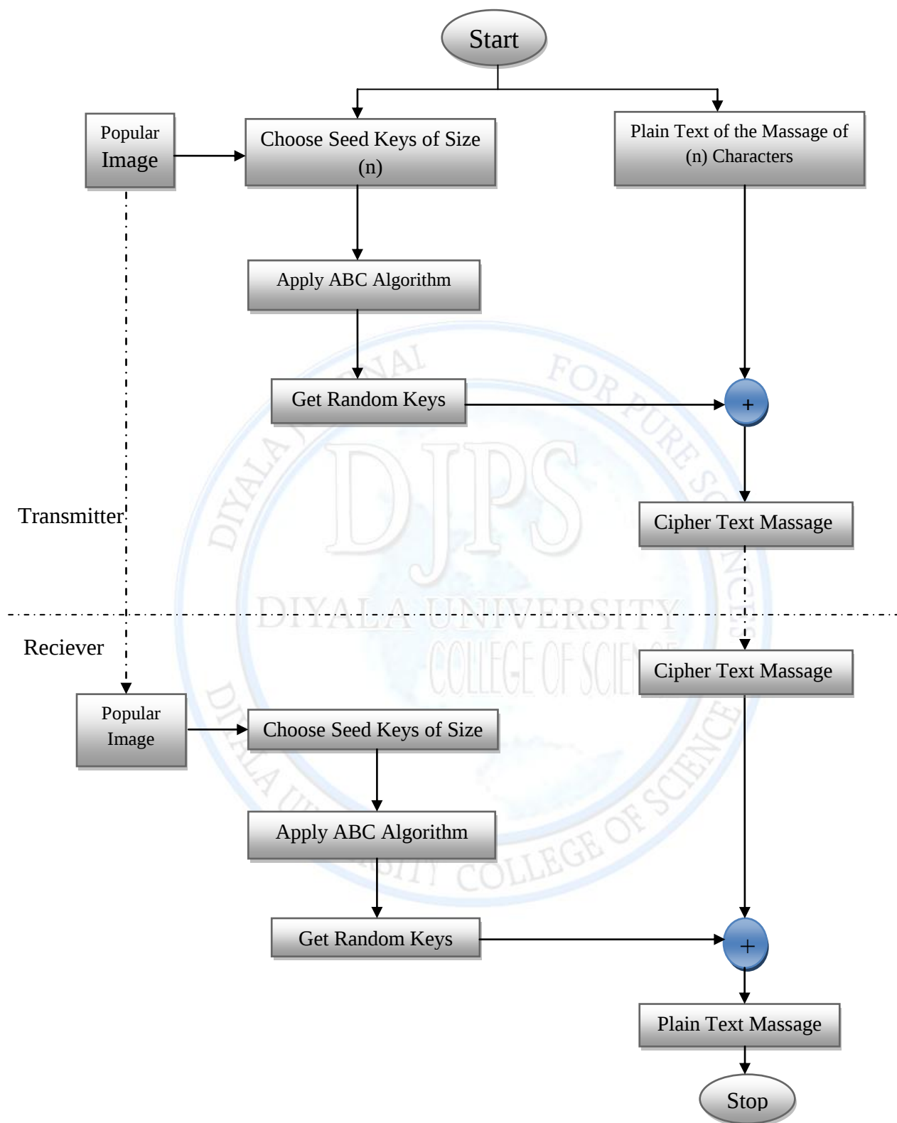
Figure (2) Block Diagram of the Proposed System
