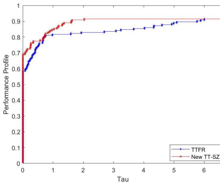
Figure (4.1): ITER comparison between TT-SZ and TT-FR.
