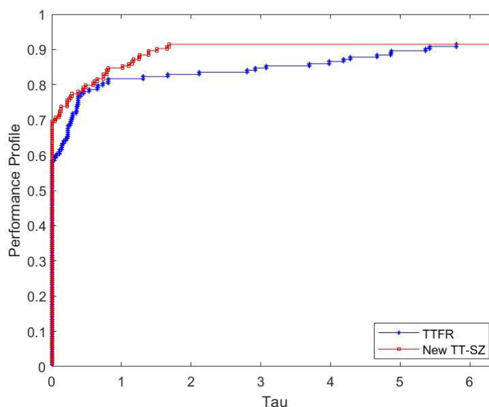
Figure (4.3): CPU comparison between TT-SZ and TT-FR.
