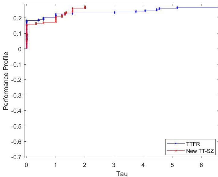
Figure (4.2): NOFG comparison between TT-SZ and TT-FR.
