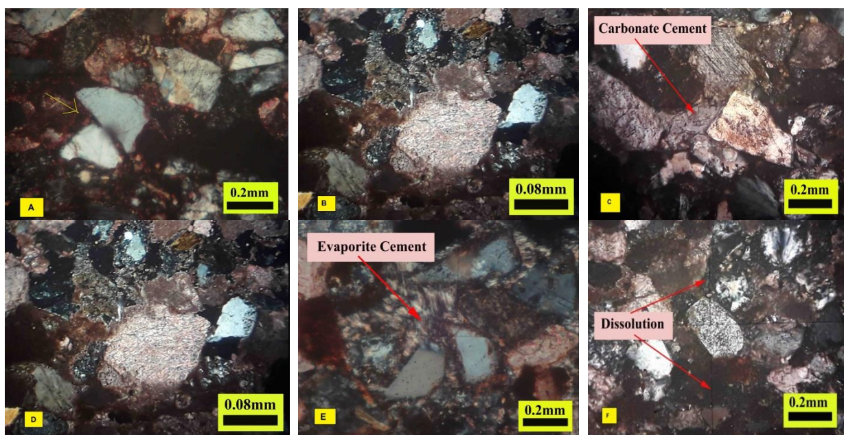
Plate 1: (A)Point&liner contact,(B)Low degree of curvature (C)Carbonate cement and blocky spary calcite,(D)Iron oxide cement,(E) Evaporite cement,(F) Dissolution process
