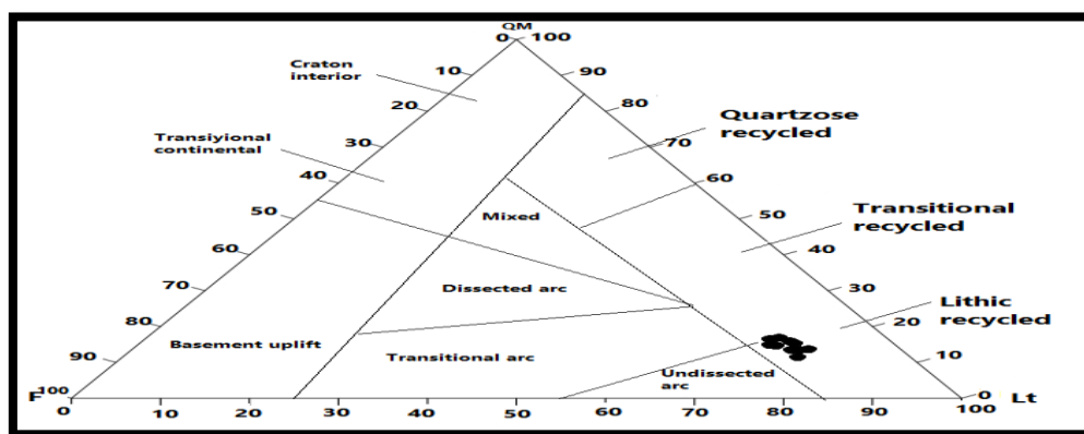
Fig. 6: QmFLt Injana samples in both sections from the field placed with recycled lithic zone according to the QmFLt diagram.
