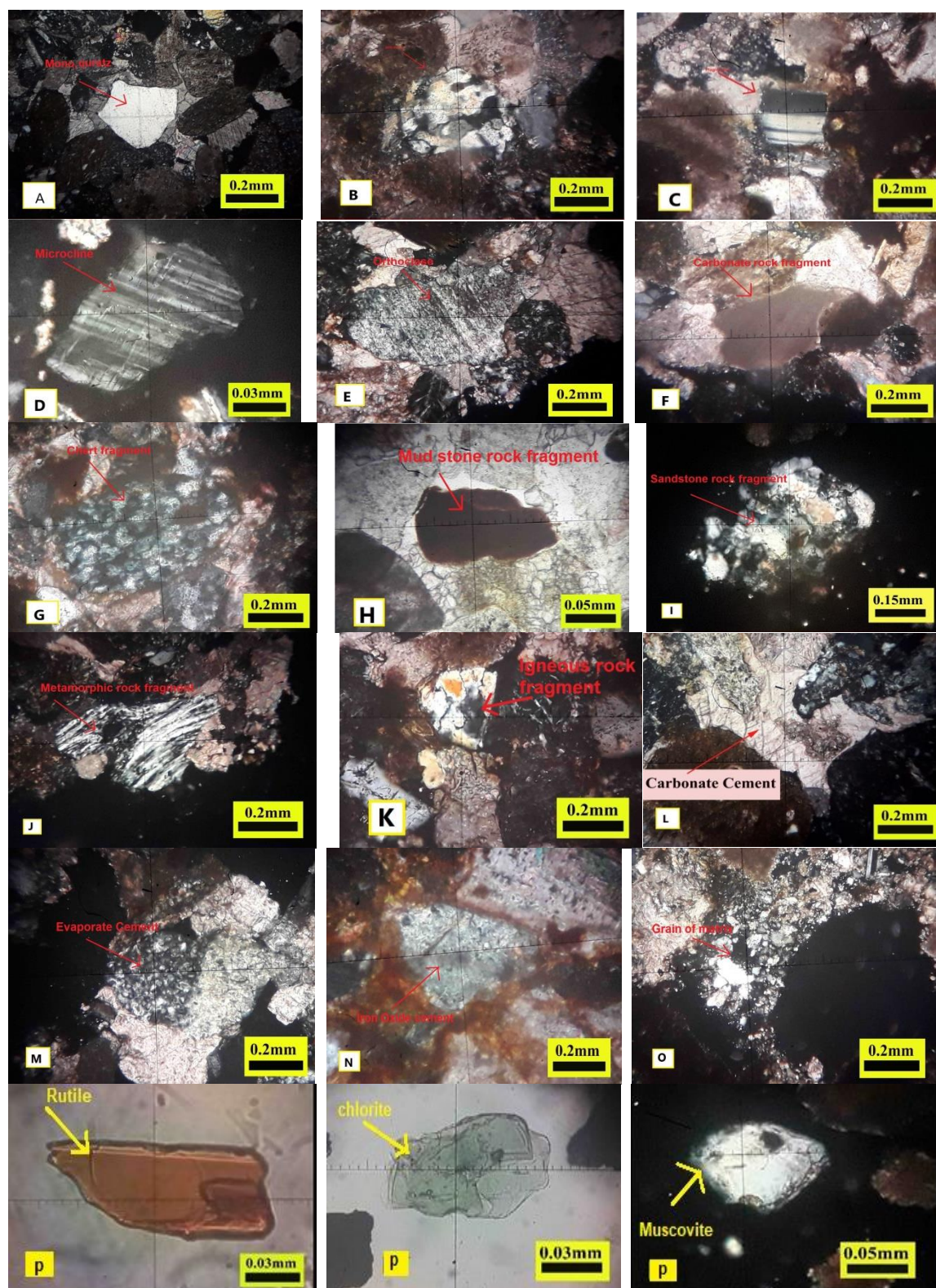
Fig. 4: Crossed Nicol (XPL) photomicrograph of Injana sandstone detrital grains at The Zawita and Dekala region, demonstrating: A: mono. quartz, B: poly. quartz, C: plagioclase, D: microcline, E: orthoclase, F: carbonate rock fragments, G: Chert fragments and H: Mud Stone rock fragments, I: Sandstone rock fragments, J: Metamorphic rock fragments, K: Igneous rock fragments, L: Carbonate cement, M: Evaporate cement, N: Iron Oxide cement, O: Grain of Matrix and P: Other Component
