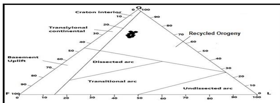
Fig. 7: QFL injana samples in both sections in recycled orogens are the original tectonic source of studied samples that produced via the up folding or up faulting of sedimentary or metasedimentary terrains, enabling the recycling of the rock debris into associated basins.
