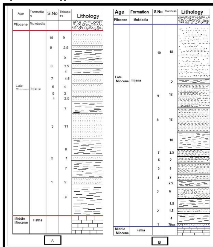
Fig. 3: Sedimenological section of Injana Formation at Dekala area (A) and Zawita area (B).
