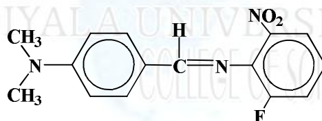
N-(4-(dimethylamino)benzylidene)-2-fluoro-6-nitroaniline
