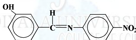
3-((4-nitrophenylimino)methyl)phenol
