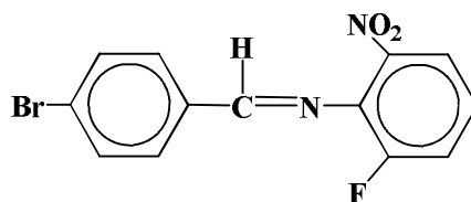
N-(4-bromobenzylidene)-2-fluoro-6-nitroaniline
