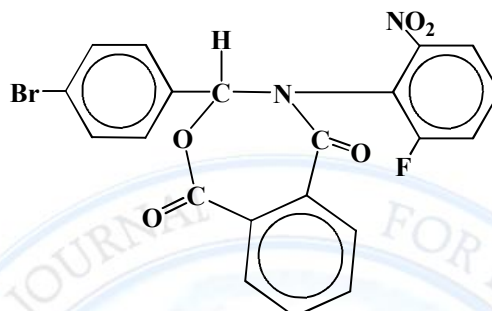
3-(4-bromophenyl)-4-(2-fluoro-6-nitrophenyl)-3,4-dihydrobenzo[e][1,3]oxazepine-4,7-dione
