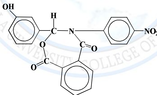
3-(3-hydroxyphenyl)-4-(4-nitrophenyl)-3,4-dihydrobenzo[e][1,3]oxazepine-4,7-dione
