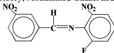
2-fluoro-6-nitro-N-(3-nitrobenzylidene)aniline
