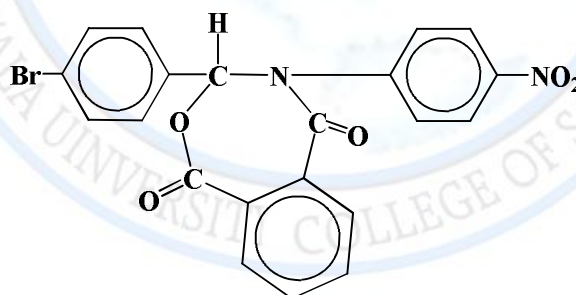
3-(4-bromophenyl)-4-(4-nitrophenyl)-3,4-dihydrobenzo[e][1,3]oxazepine-4,7-dione
