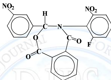
4-(2-fluoro-6-nitrophenyl)-3-(3-nitrophenyl)-3,4-dihydrobenzo[e][1,3]oxazepine-4,7-dione
