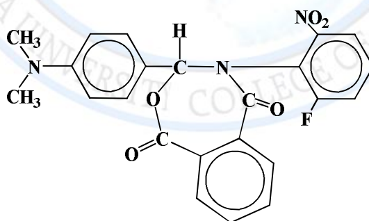
3-(4-(dimethylamino)phenyl)-4-(2-fluoro-6-nitrophenyl)-3,4-dihydrobenzo[e][1,3]oxazepine-4,7-dione
