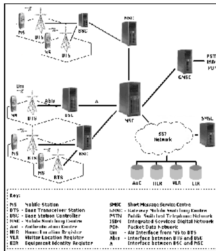
Figure. 1. GSM Architecture (adapted from [12])
