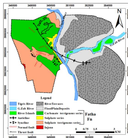
Fig. 2: Geological map of the study area [1]
