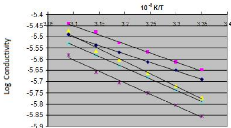
Fig(4) : Log Conductivity verse T^{-1} for CTC (1-5) with DDQ in C_2H_4Cl_2
